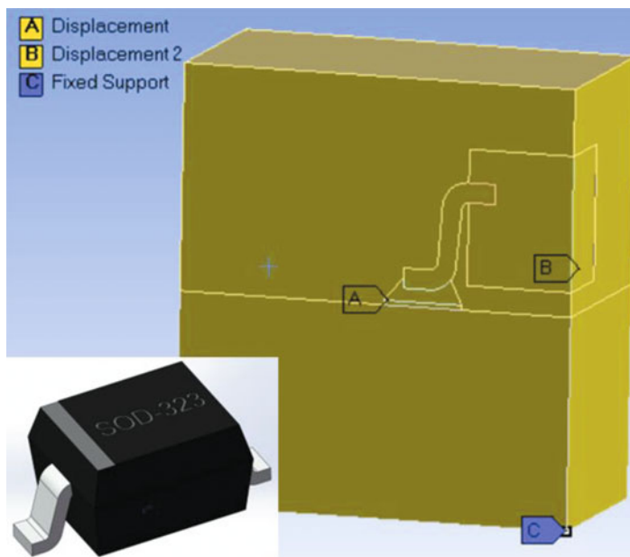
Fig. 13.6 Schematic of a quarter of SOD323 model used in FEM and boundary condition
