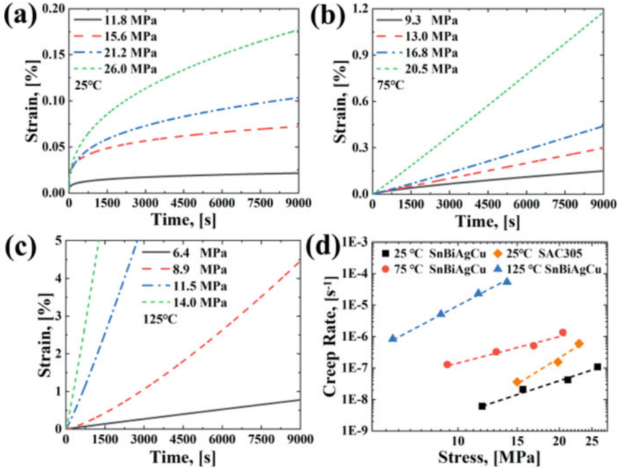
Fig. 13.4 Creep curves of solder alloys under different temperatures: (a) SnBiAgCu, 25 °C; (b) SnBiAgCu, 75 °C; (c) SnBiAgCu, 125 °C; and (d) creep rate of SnBiAgCu and SAC305
