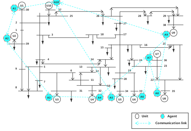
Fig. 9: IEEE 39-bus system.
