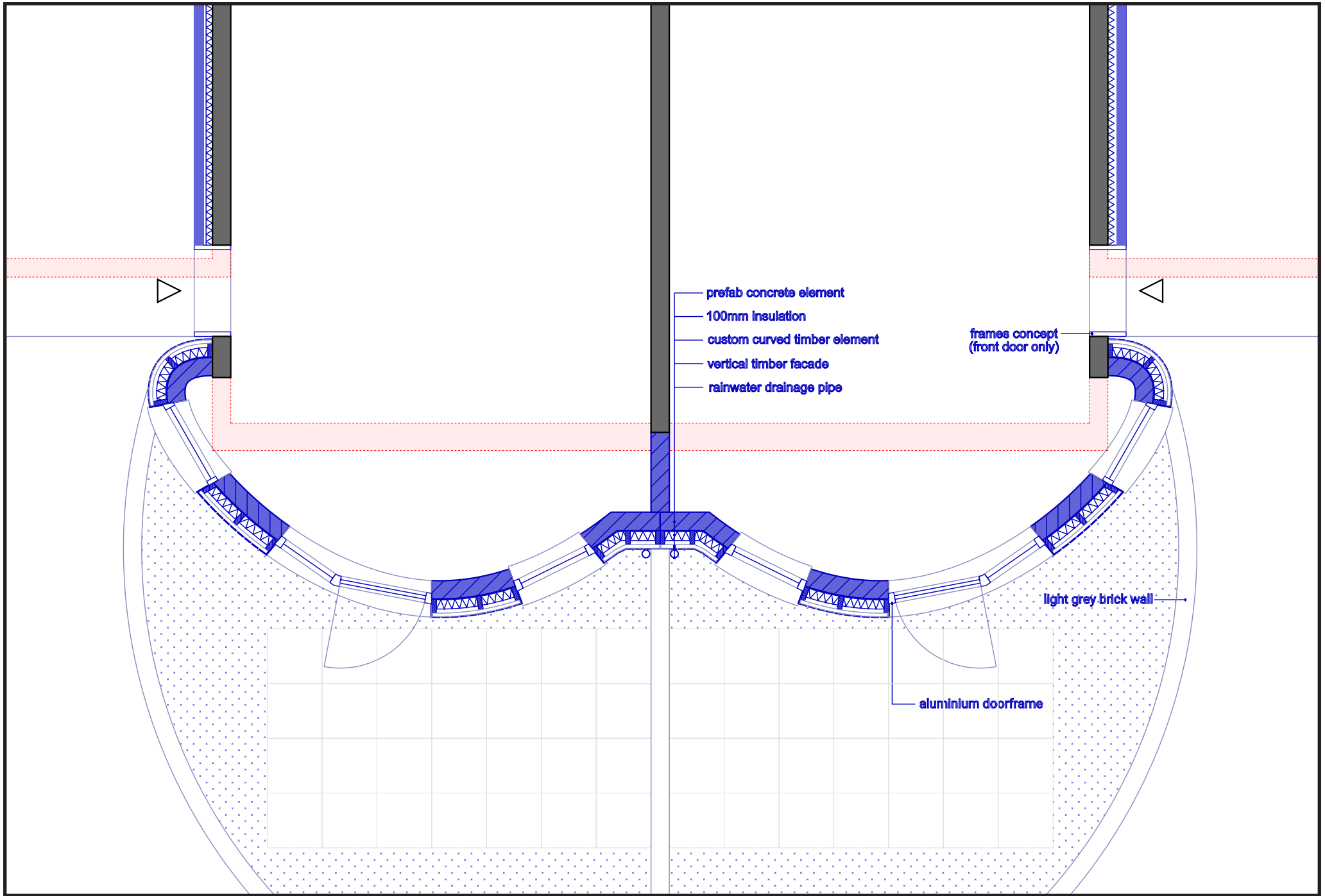
Facade fragment, horizontal cross-section
