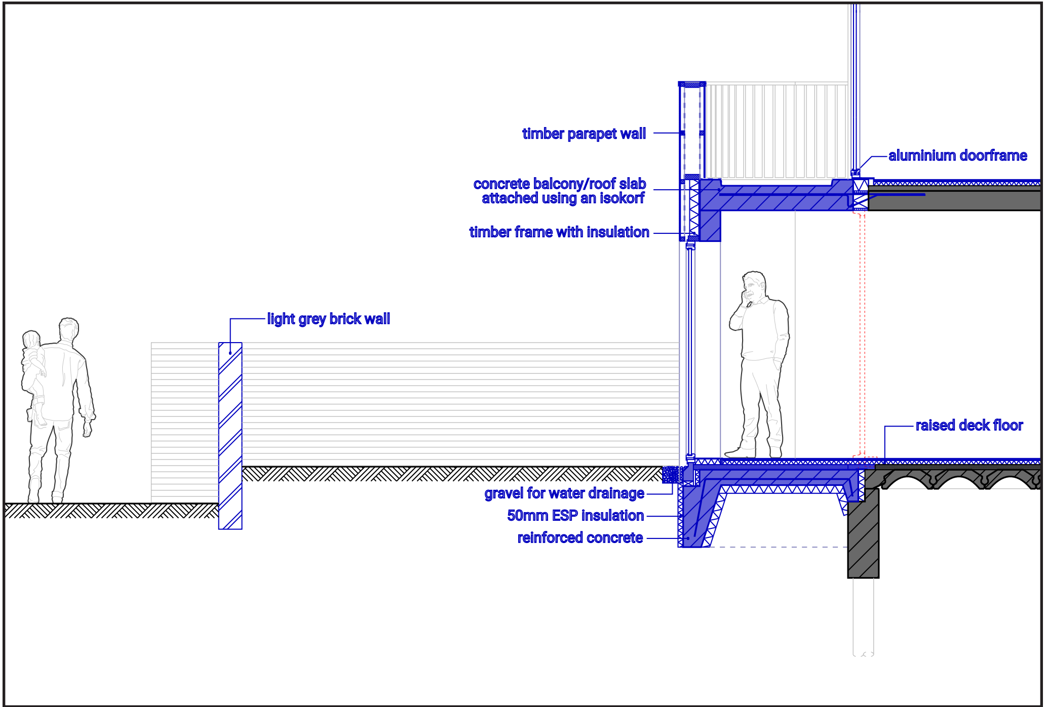
Facade fragment, vertical cross-section
