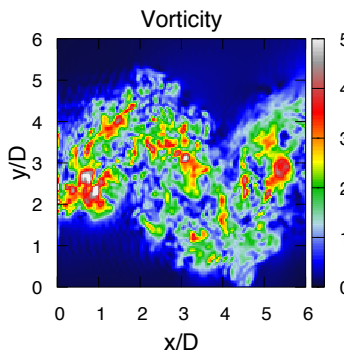
Figure 22: Instantaneous flow vorticity in the streamwise plane z = 1.31D calculated from the true observations.
