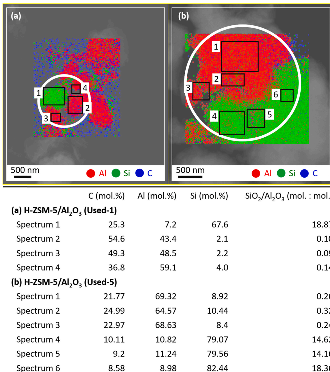
Fig. 7. Elemental (Al and Si) maps of the used H-ZSM-5/Al 2 O 3 catalysts. (The white circle represent holes in the carbon-coated copper grid).
