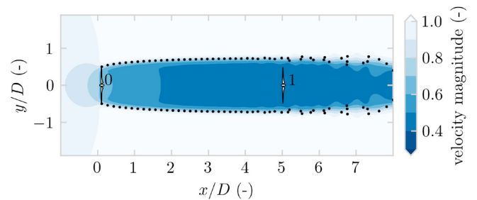
Fig. 1. Illustration of a flow field at hub height with the wind turbine wake for turbine 0, where turbine 1 at x/D = 5 downstream is modelled using the effective flow velocity. Units have been non-dimensionalised by rotor diameter and inflow velocity magnitude. The vortex points used for the velocity calculation are marked with black dots.
