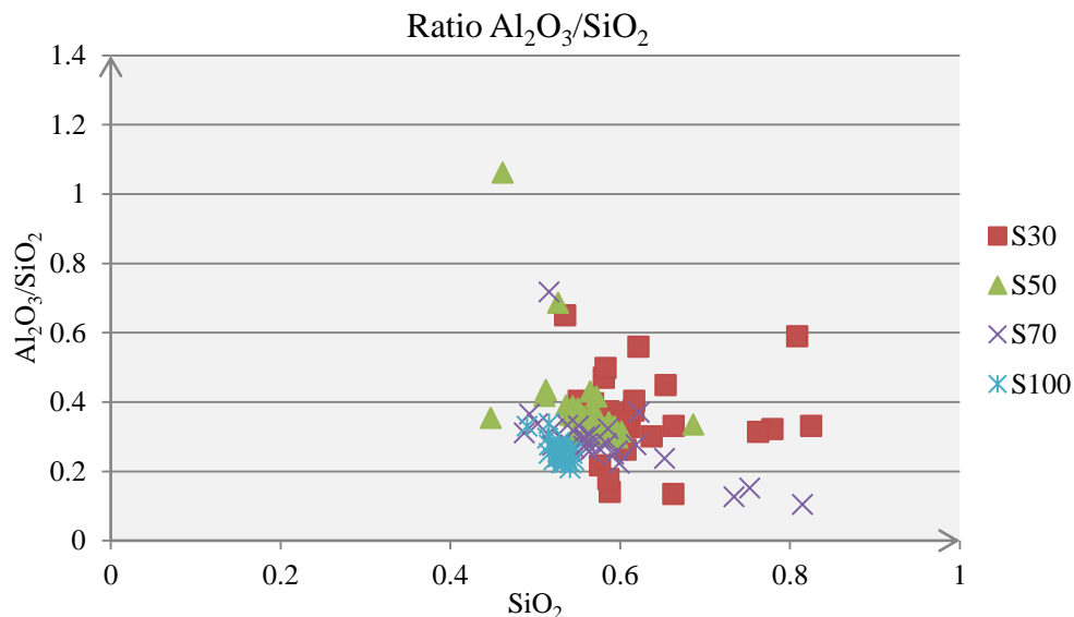
Figure 4: \text{SiO}_2 vs \text{Al}_2\text{O}_3/\text{SiO}_2 for alkali activated pastes at 28 days
