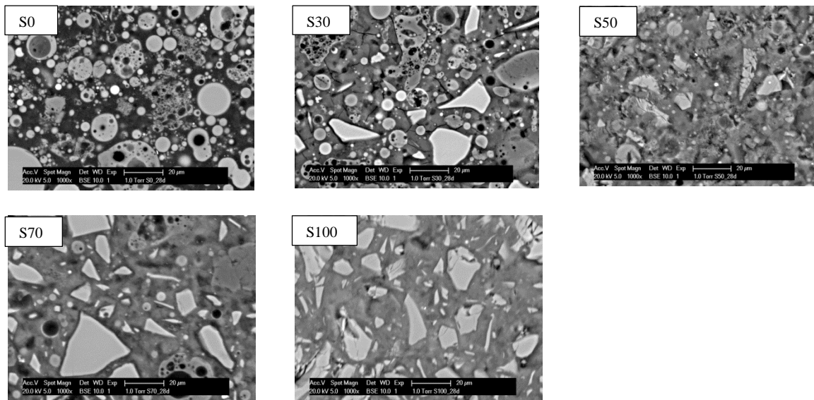
Figure 8: BSE images of alkali activated pastes at 28 days
