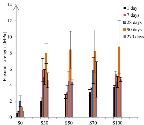
Figure 2: Flexural strengths of alkali activated fly ash/slag pastes at different ages
