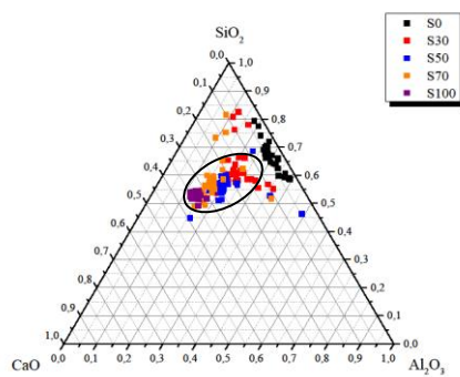
Figure 9: Ternary diagram of CaO-Al 2 O 3 -SiO 2 as a function of slag replacement level
