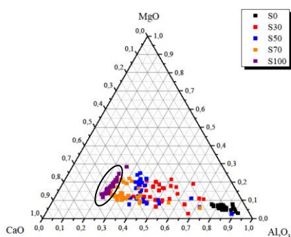
Figure 10: Ternary diagram of CaO-Al 2 O 3 -MgO as a function of slag replacement level
