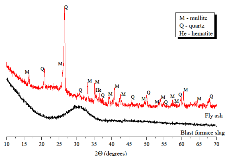
Figure 1: XRD patterns of unreacted FA and BFS
