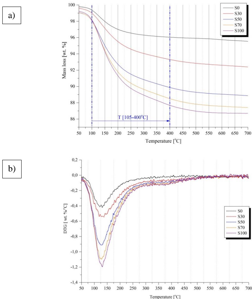
Figure 7. TGA spectra (a) and DTGA (b) of the alkali activated fly ash and slag pastes at 28d
