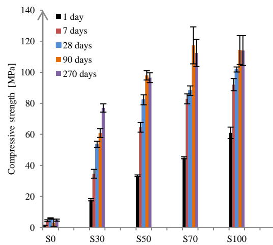
Figure 3: Compressive strengths of alkali activated fly ash/slag pastes at different ages
