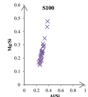
Figure 11: Atomic Mg/Si vs Al/Si for alkali activated pastes at 28 days
