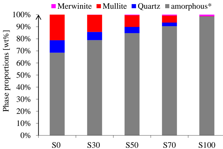
Figure 6. XRD quantification of different phases formed in S0, S30, S50, S70, S100, respectively at 28 days
