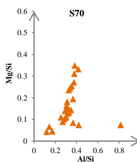
Figure 11: Atomic Mg/Si vs Al/Si for alkali activated pastes at 28 days
