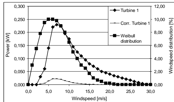
Figure 8: The Weibull wind speed distribution at the island of Texel, the wind speed converted generator response of Turbine 1 and the power correlation between wind speed distribution and turbine performance.
