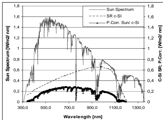
Figure 6: The sun's spectrum at sea level, the spectral response (SR) of a crystalline silicon (c-Si) PV cell and the power correlation between the Sun spectrum and a c-Si PV cell [1].
