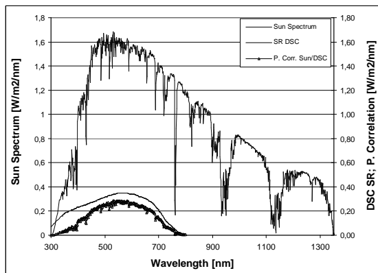
Figure 7: The sun's spectrum at sea level, the spectral response (SR) of a Dye Sensitized (DSC) PV cell and the power correlation between the Sun spectrum and a DSC PV cell. [1].
