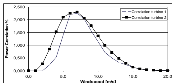
Figure 10: Comparison between the power correlation of Turbine 1 and 2.
