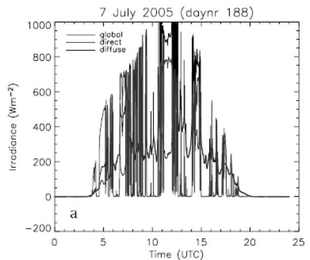
Figure 13: Measurements of sunlight at de Bilt in the Netherlands (in W/m^2 ) of direct normal, diffuse and global irradiance as function of time during one day on 7 th of July 2005 [9].
