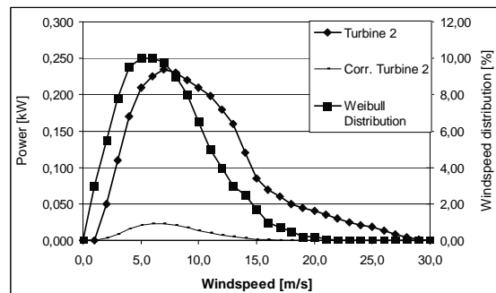
Figure 9: The Weibull wind speed distribution at the island of Texel, the wind speed converted generator response of Turbine 2 and the power correlation between wind speed distribution and turbine performance.
