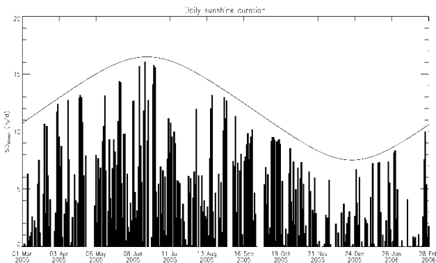
Figure 11: Daily sunshine duration (h) according to the direct method (bars) and the maximum possible sunshine duration (solid line) in one year [9]
