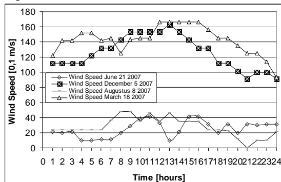
Figure 12: Seasonal variations in wind speed during one year, measured at the northern provinces of the Netherlands [9].
