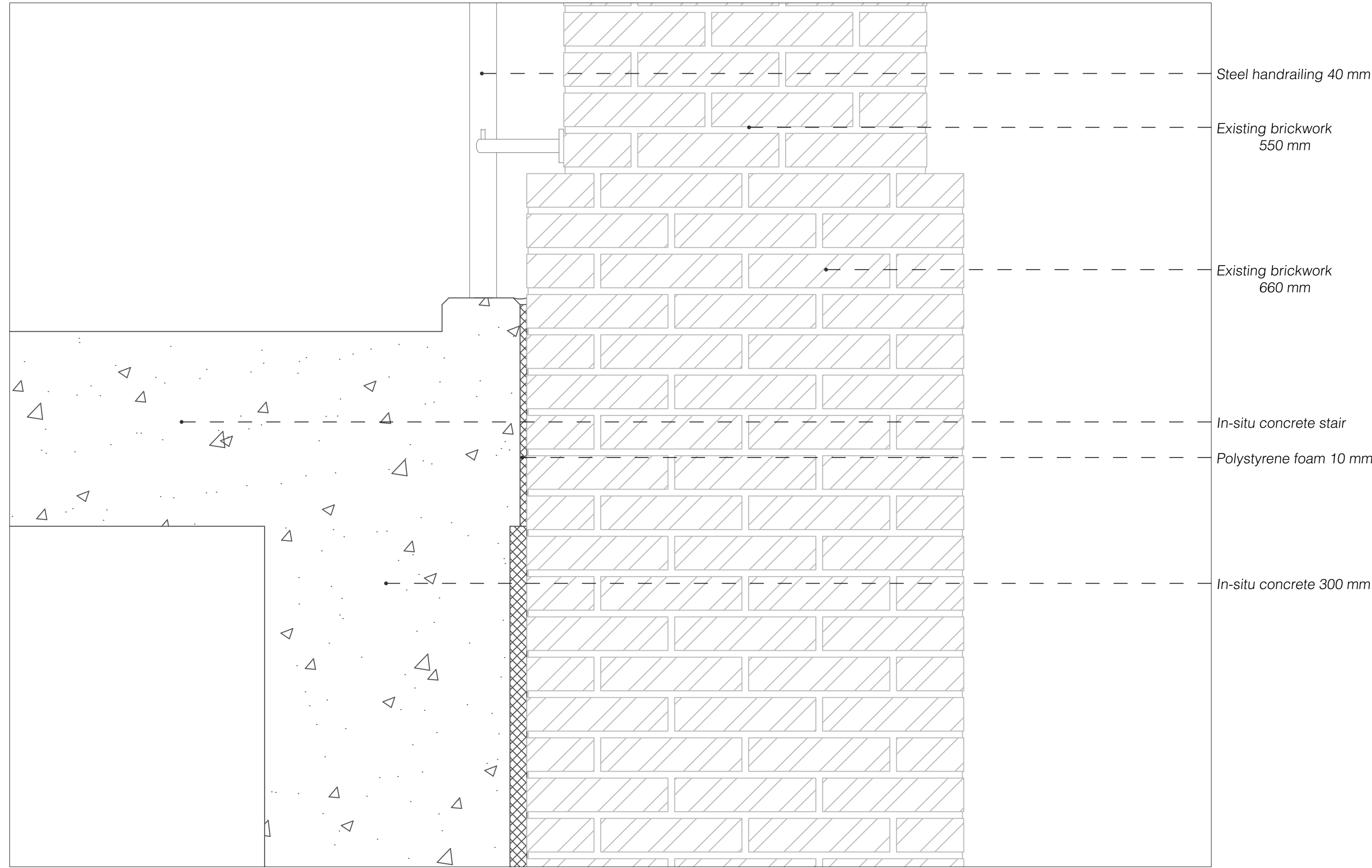
3. 1:5 Detail
