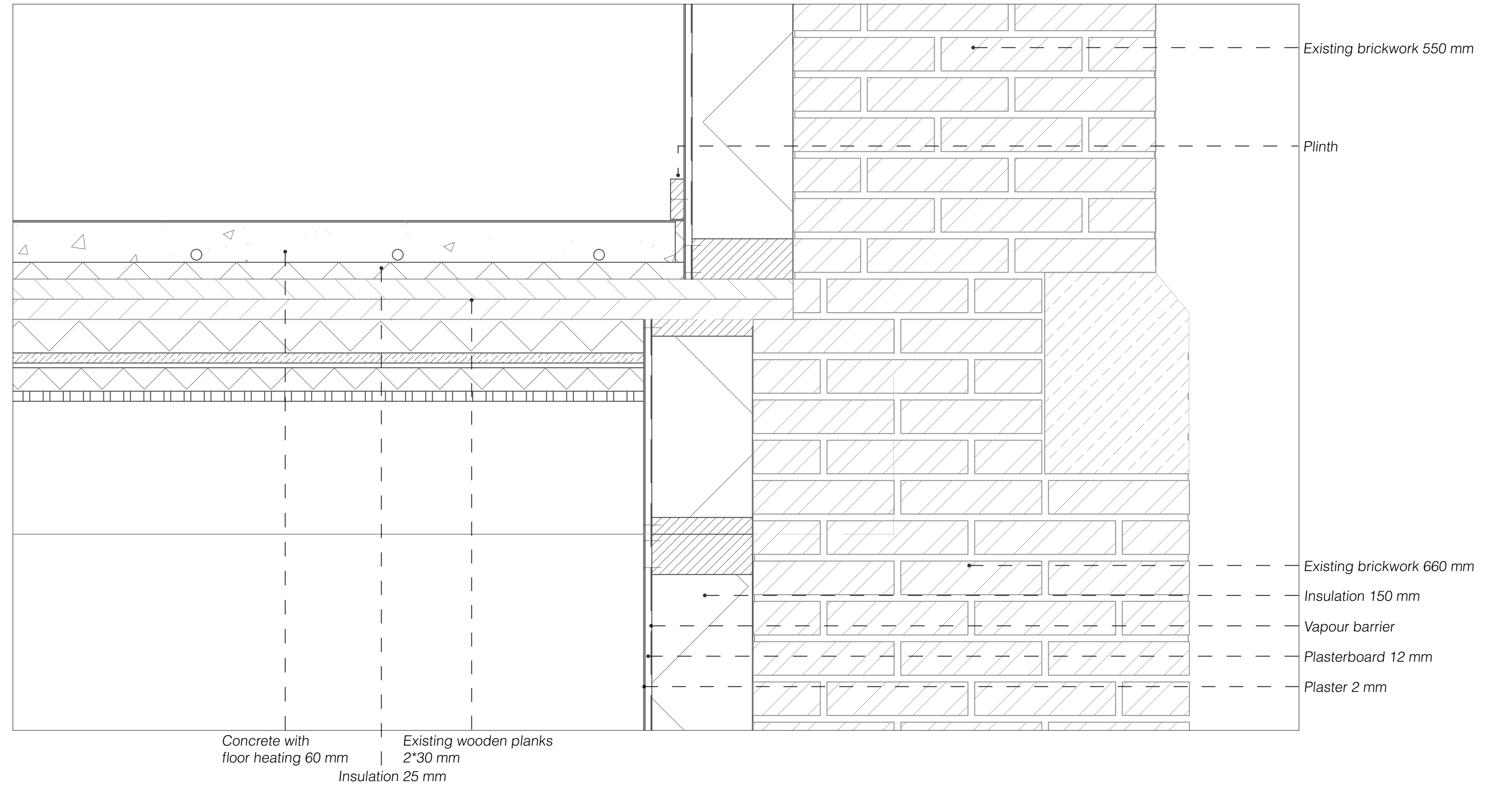
6. 1:5 Detail
