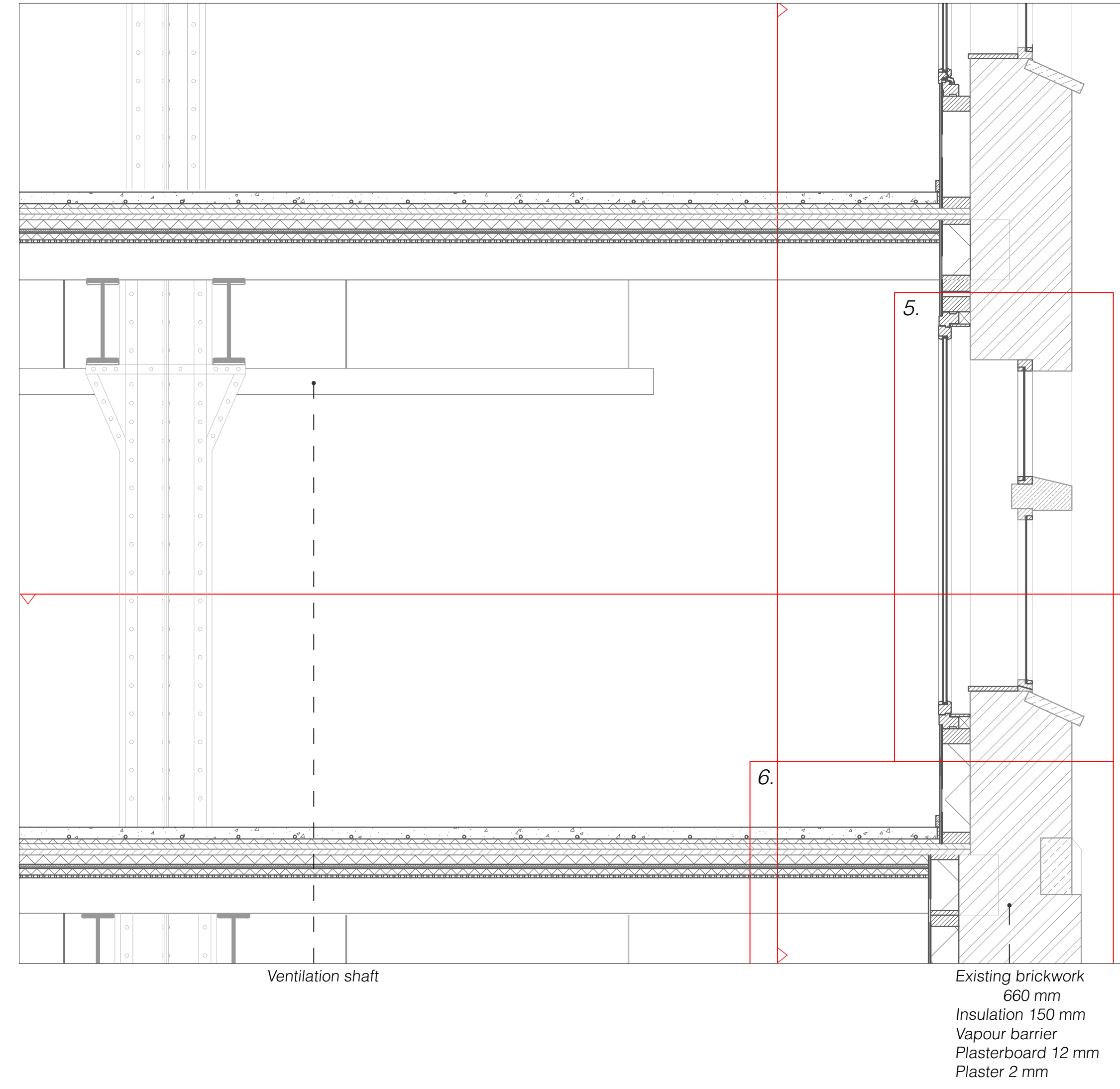
1:20 Section
