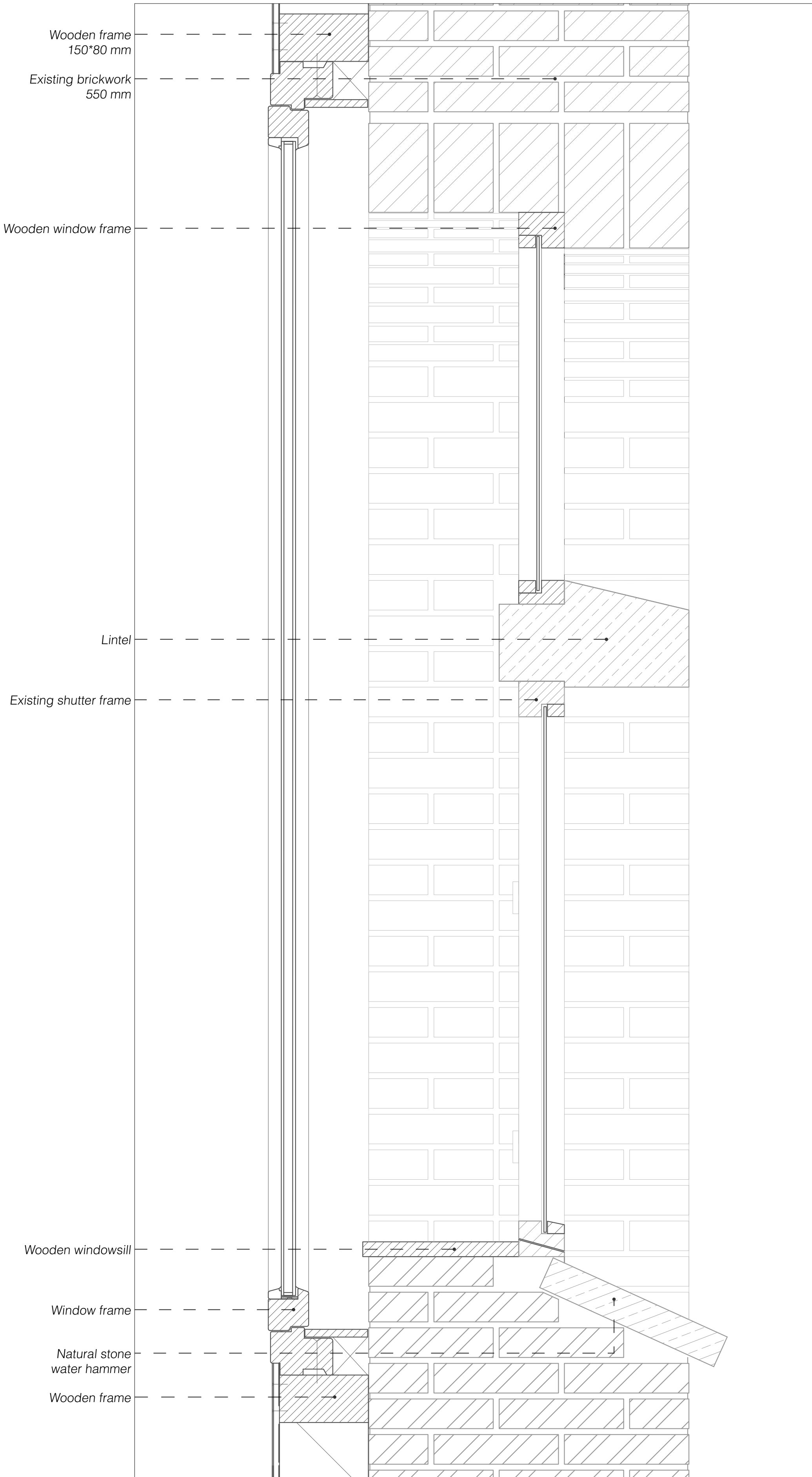
5. 1:5 Detail
