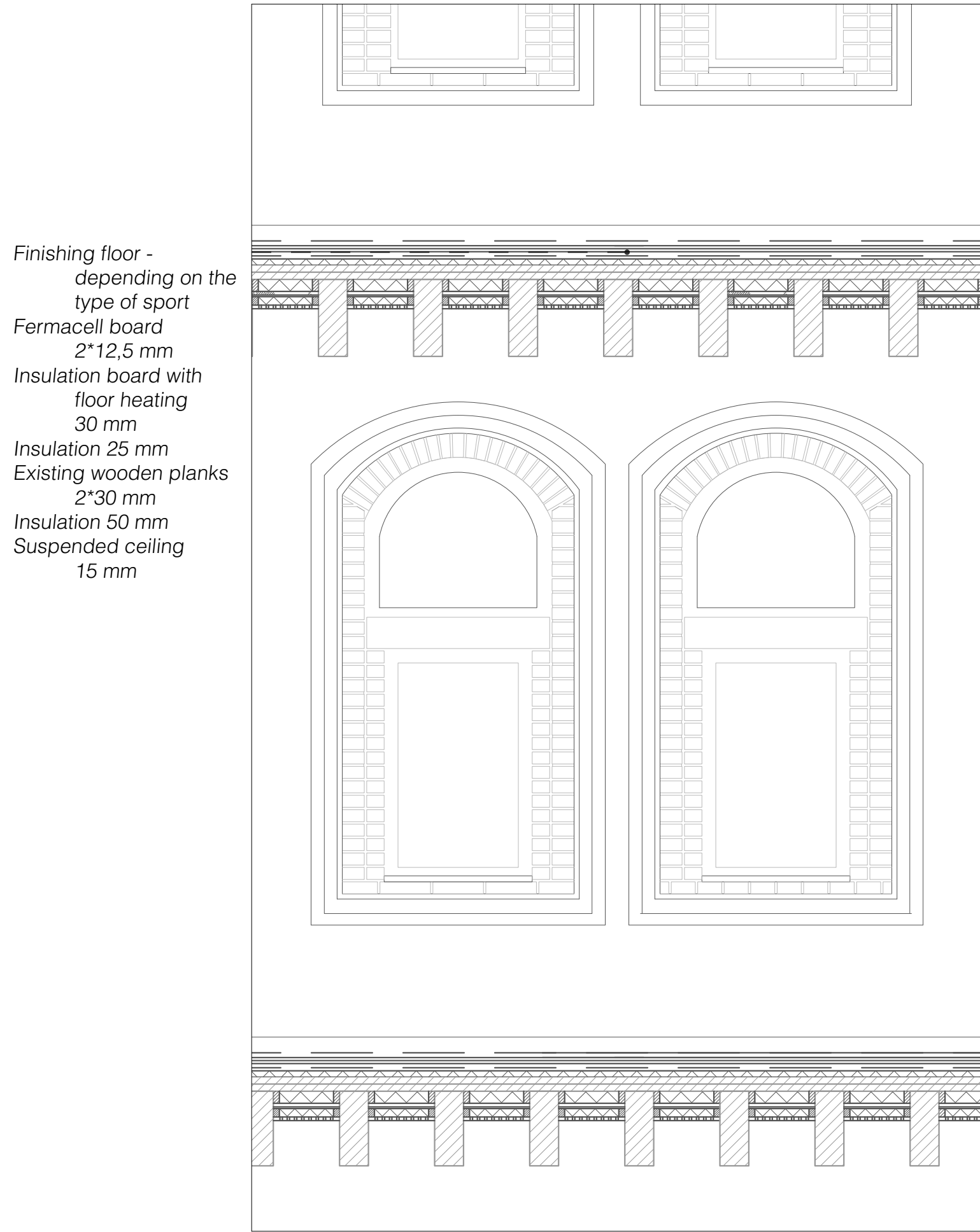
1:20 Inside elevation
