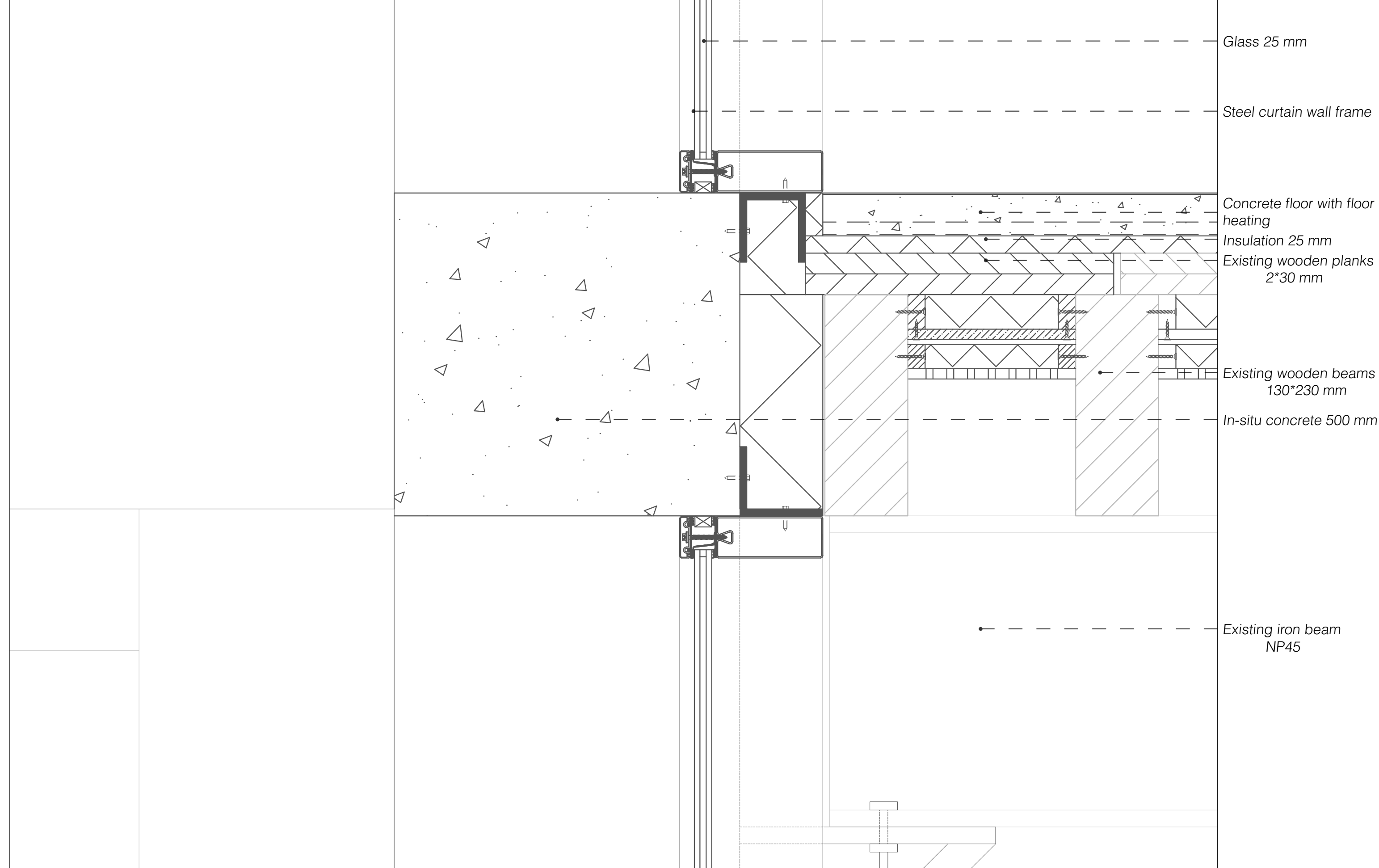
2. 1:5 Detail
