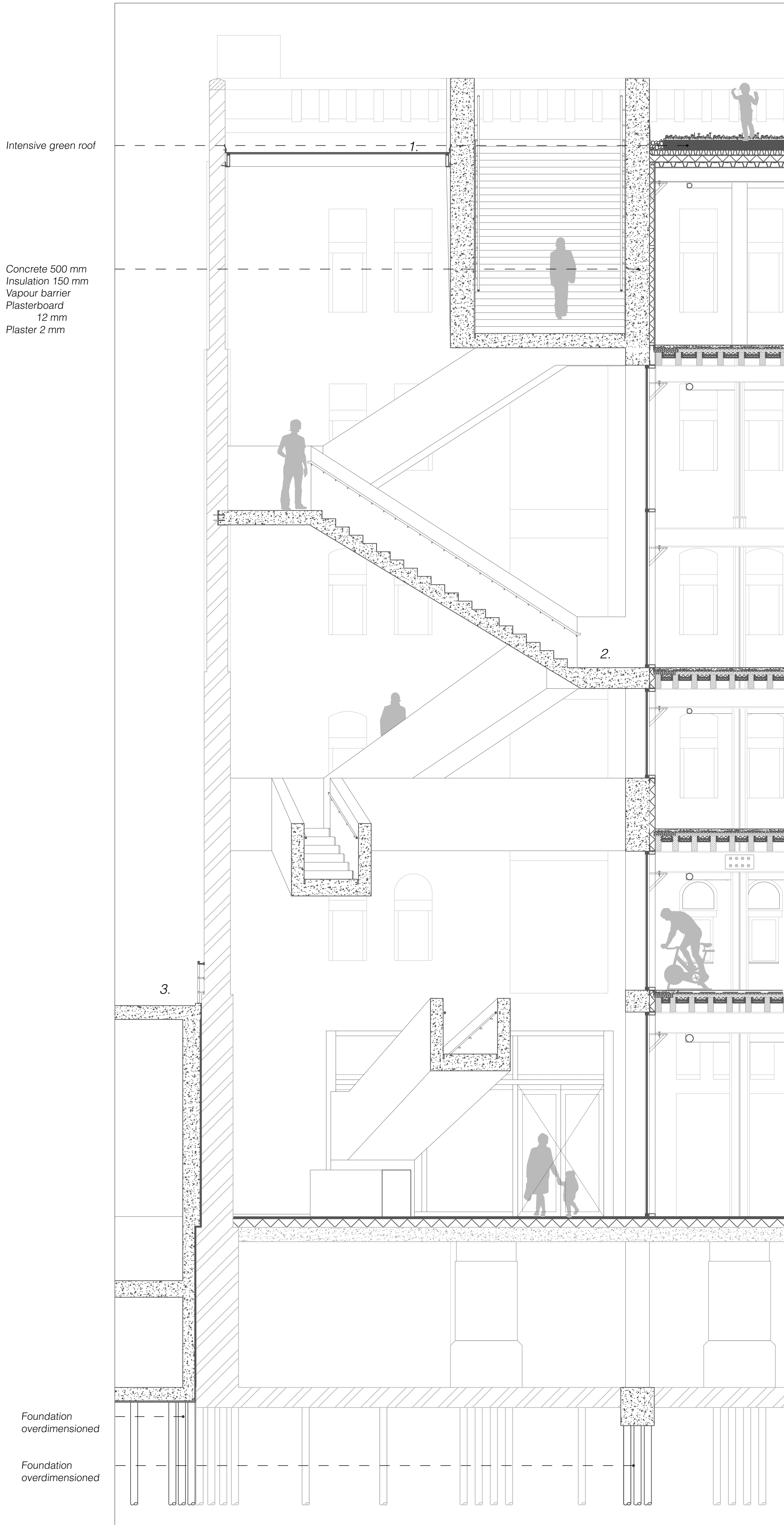
1:50 Section
