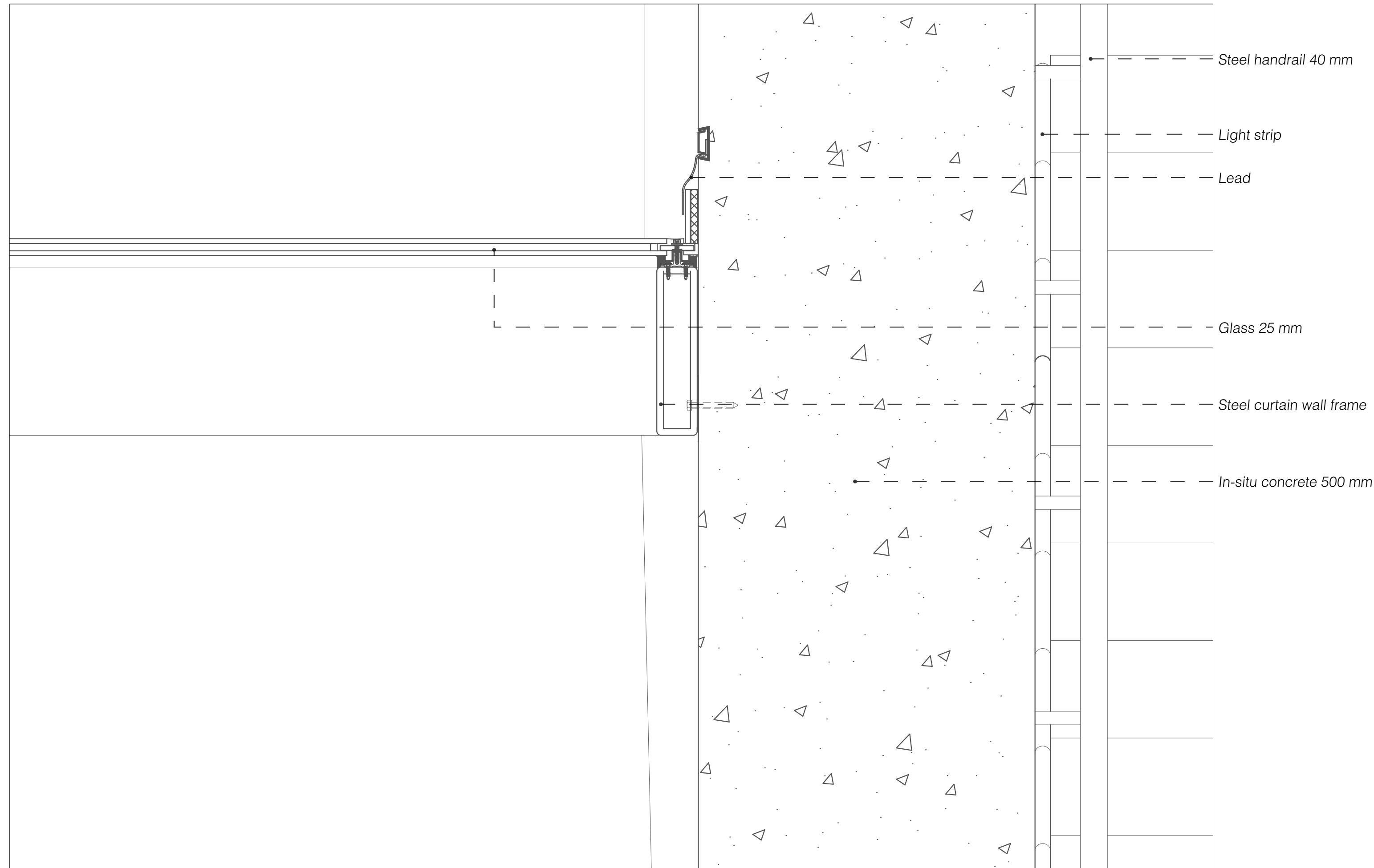
1. 1:5 Detail
