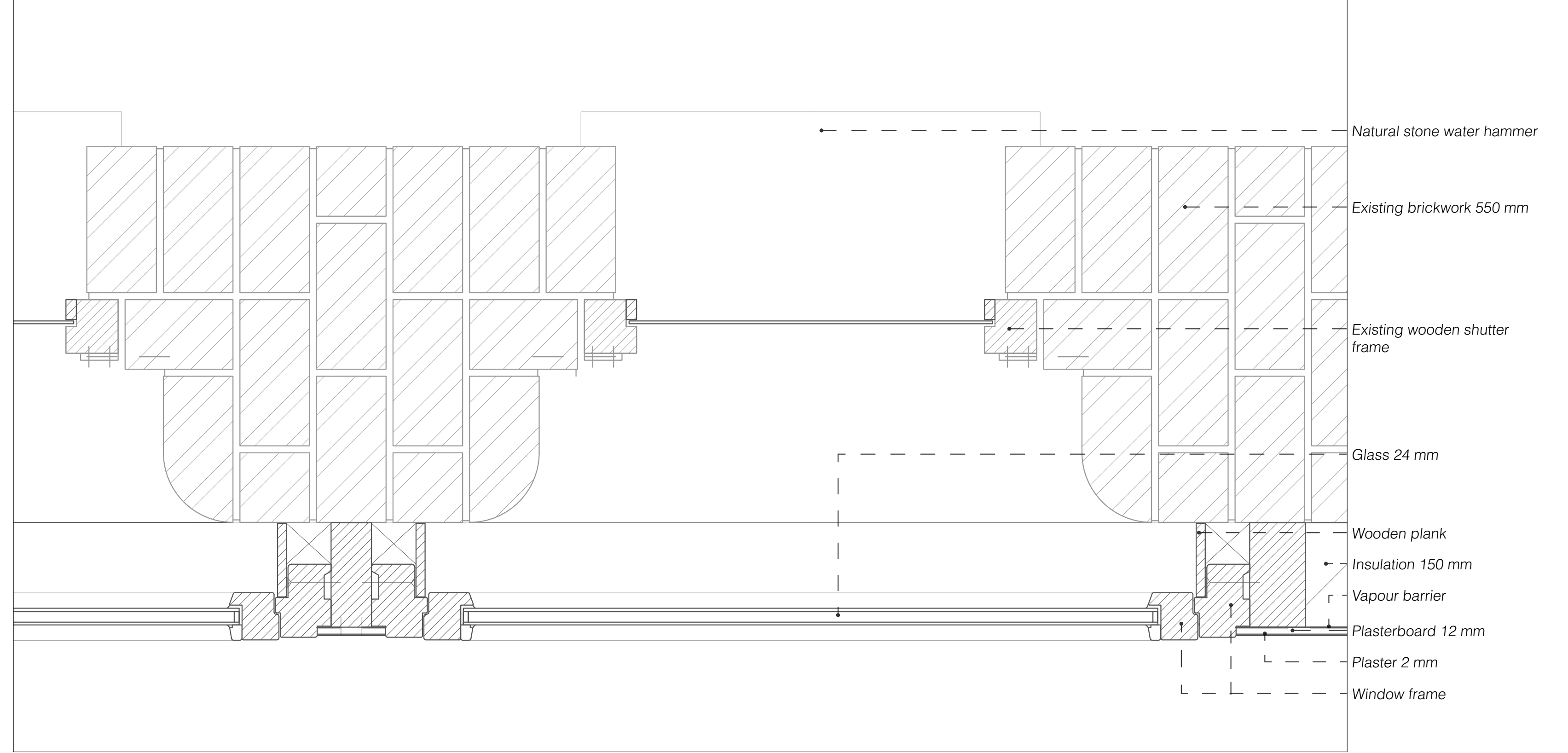
7. 1:5 Detail
