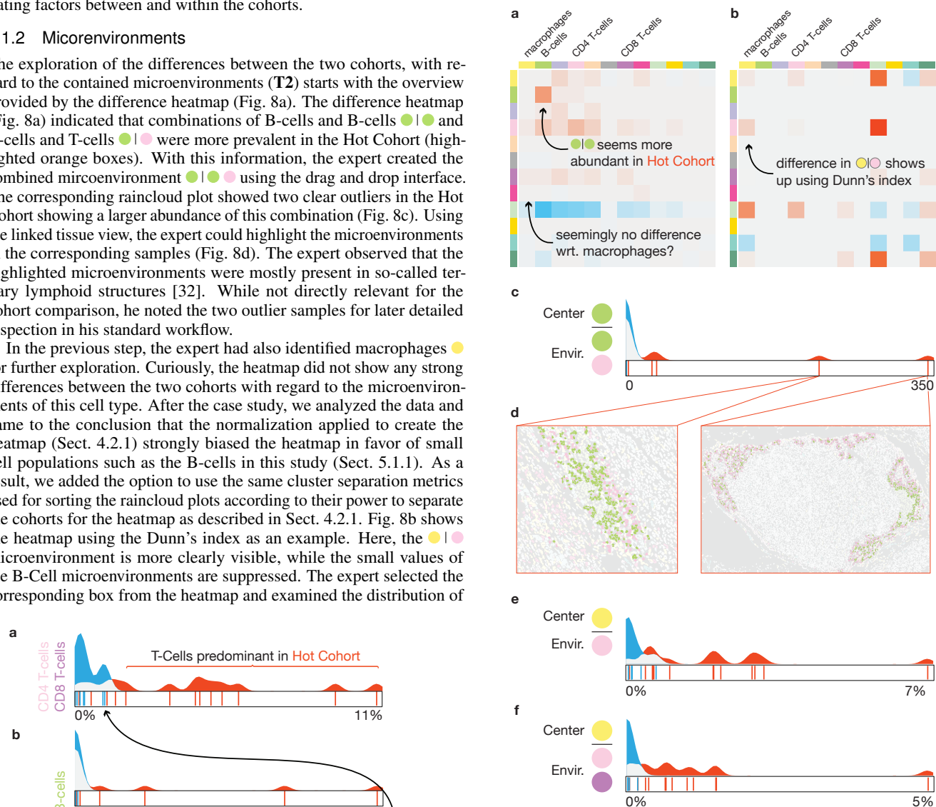
Fig. 8. Multi-cellular microenvironment cohort comparison. (a) A heatmap depicting the difference of the amount of pairwise spatial interaction between two cohorts normalized according to the abundance of each cell type. (b) A heatmap depicting the Dunn index for the samples of each cohort for each pairwise co-localization pattern. (c) The amount of B-cells having in their microenvironment B-cells and CD4 T-cells, depicting that the occurred differentiation in (a) was due to the two outlier samples, which exist in a tertiary lymphoid structure, an interesting biological structure (d). The amount of macrophages having in their microenvironment CD4 T-cells (e) and CD8 T-cells (f).
