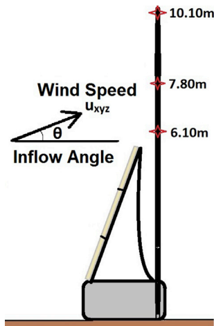
Fig. 10. Wind speed U_{xyz} (m/s) magnitude vector and the inflow angle \theta^{(0)} , illustrated for a perpendicular flow indicating the presence of sonic anemometers with red stars in different heights for Pole 1. (For interpretation of the references to colour in this figure legend, the reader is referred to the Web version of this article.)
