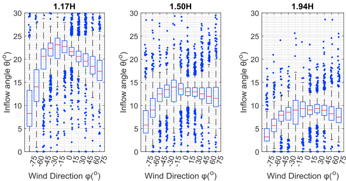
Fig. 13. Box plots of 3 different heights of the 10-min averaged inflow angle \theta(^{\circ}) for different wind directions \varphi(^{\circ}) .
