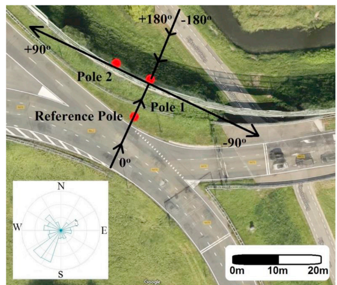
Fig. 3. Top view of the studied noise barrier (bottom left) Wind orientation rose (red circles filled in black) Poles with the sonic anemometers (black lines and arrows) The reference system used in this study. (For interpretation of the references to colour in this figure legend, the reader is referred to the Web version of this article.)
