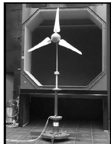
Fig. 6. (Right) Micro wind turbine placed in front of the nozzle of Open Jet Facility in TU Delft (left) plan drawing of the distances.
