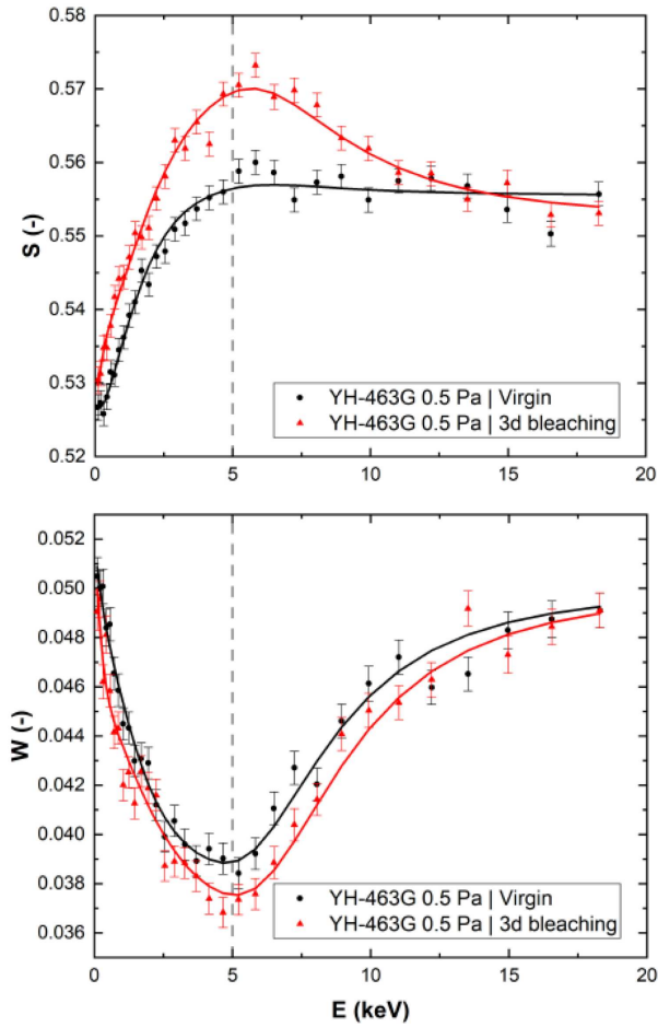
Fig. 2. Positron Doppler broadening S - and W -parameter depth-profile of the 330 nm YO_xH_y sample in (i) the as-deposited virgin state (black circles) and (ii) the state after 2 h of UV-illumination and 3 days of bleaching during the in situ PAS measurements (red triangles).
