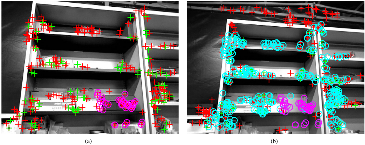
Figure 3: A database image (a) and a query image with one object missing on the third shelf from the top (b). The crosses represent the features in both images. Tentative correspondences found by the matching algorithm are shown in green. The cyan circles show the transformations of the features from the database image to the query image. The magenta circles show the features that were identified as a change.
