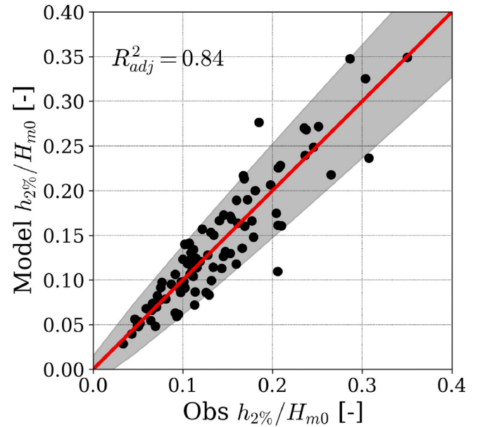
Fig. 9. Comparison of measured (Obs) and estimated (Model) h_{2\%}/H_{m0} using Eq. (25). The gray band show the 90% confidence using a and b for Eq. (22) given by 0.0057 and 0 respectively.
