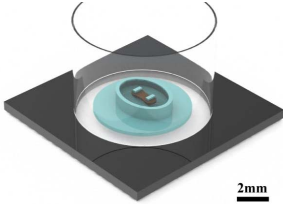
Fig. 1. A 3D model of the miniaturized EHT platform: a PDMS layer (blue) on the bottom of a cell culture well with the tissue (brown) formed around two pillars and confined by an elliptical sub-well. The transparent ring around the structure represents a single unit of a standard 96-well tissue culture plate.
