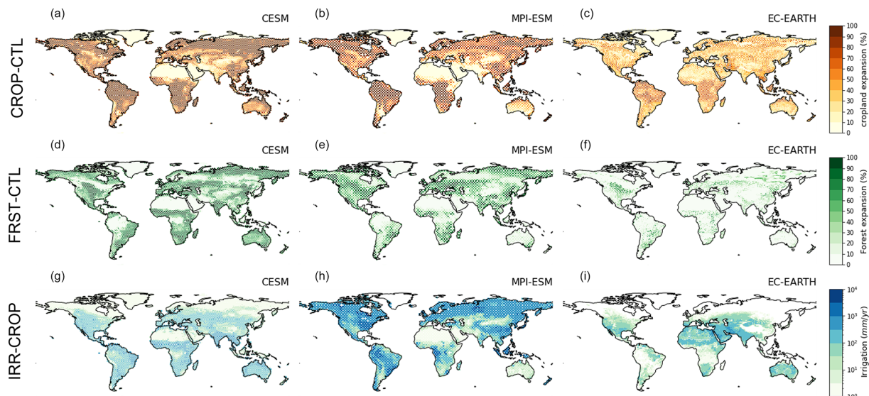
Figure 1. Land cover and land management changes as implemented in the three different ESMs. Cropland expansion (CROP-CTL; a–c), afforestation (FRST-CTL; d–f), and irrigation expansion (IRR-CROP; g–i) implemented in CESM, MPI-ESM, and EC-EARTH, respectively. Both cropland expansion and afforestation are shown as a change in area fraction (%), while irrigation expansion is shown through the irrigation flux (in \text{mm yr}^{-1} ).
