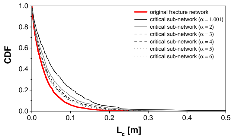
Figure 3.6 Cumulative distribution function (CDF) for the characteristic radius of matrix blocks L_c formed by the original fracture network (the bottom curve) and the dominant sub-network: power-law aperture distributions with \alpha = 1.001 - 6 . The results of one realization are shown for each value of \alpha .
