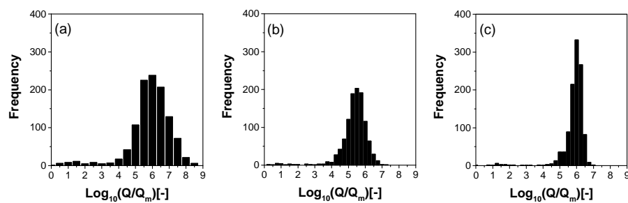
Figure 2.6 Histogram of Q for each fracture normalized by the minimum value of Q for all fractures in the backbone ( Q_m ) in log-10 space: power-law aperture distributions with (a) \alpha = 1.001 , (b) \alpha = 2 , (c) \alpha = 6 . Results of one realization shown for each value of \alpha .
