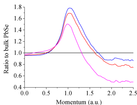
FIG. 2. The ratio curve of 1D-ACAR momentum distributions for PbSe QDs with various surface compositions: oleic acid (blue); oleylamine (red); and, EDA (magenta). All curves are normalized to the directionally averaged 1D-ACAR distribution of bulk PbSe. (a.u. = atomic units).
