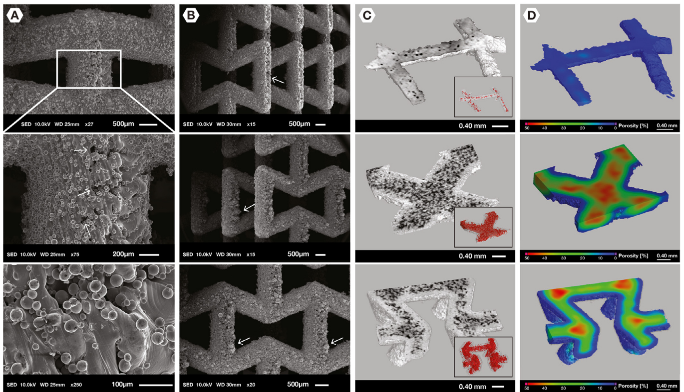
Fig. 2. (A) The structure and surface of design A (RD = 0.422) observed using SEM (27x, 75x, and 250x). (B) The structure and surface of design D (RD = 0.325) observed using SEM at 15x and 20x. (C) The inside morphology of, from top to bottom, design A (RD = 0.075), design A (RD = 0.422), and design D (RD = 0.325) imaged using micro-CT. (D) The local average porosity of, from top to bottom, design A (RD = 0.075), design A (RD = 0.422), and design D (RD = 0.325) imaged using micro-CT.
