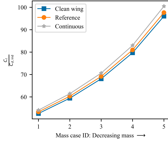
Figure 15: Comparison of C_l / C_{d,ind} for different mass cases
