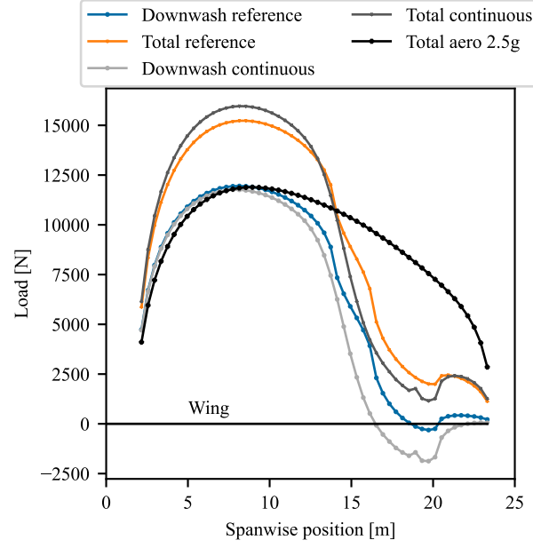
Figure 13: Lift distribution for \min(M_x) at the wing-strut attachment location during a 2.5 g pull-up
