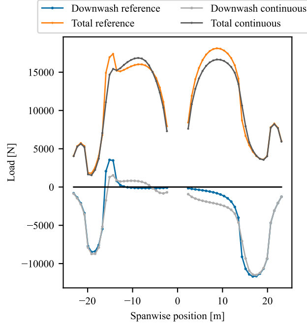
Figure 10: Lift distribution for 15 °/s roll with MLA
