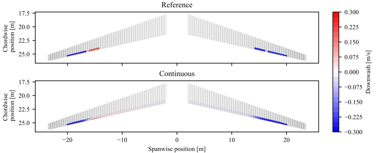
Figure 9: Downwash distribution for 15 °/s roll with MLA
