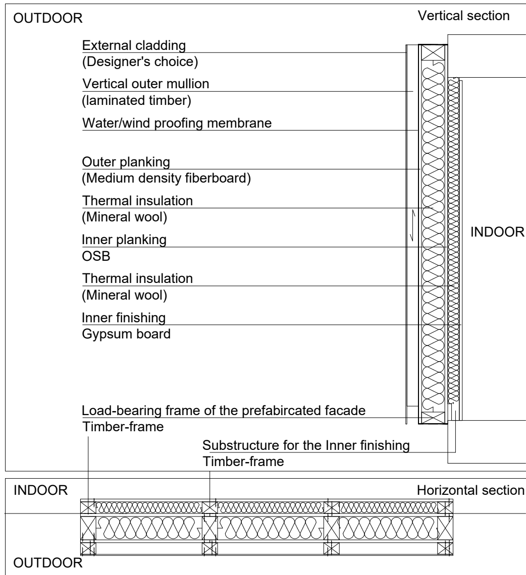
FIG. 1 Prefabricated timber-based multi-layer facade
