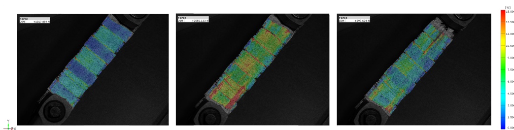
FIG. 9 Specimen 'Suntex W3' strain field along the longitudinal direction at failure (left) & directly after failure (right).
