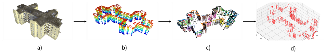
FIG. 6 a) point cloud with b) filtered window points and c) clustered windows, and d) cluster-fitted bounding boxes
