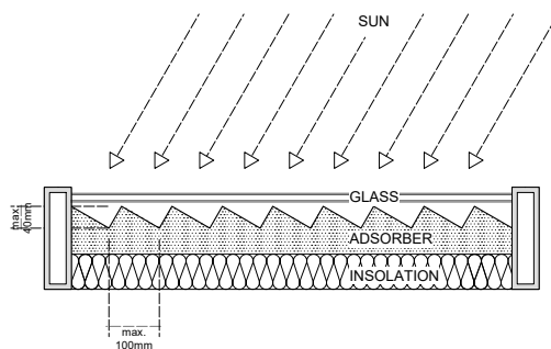
FIG. 7 Top section view of adsorption element with folded sheet
