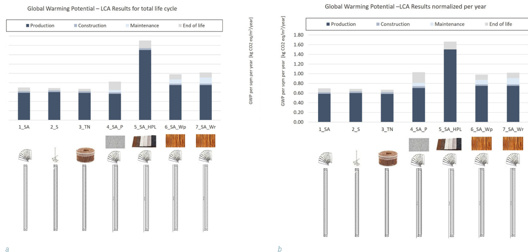
FIG. 7 Global Warming Potential (GWP) per square meter for total life cycle of different prefabricated multilayer opaque façade systems with different connection and cladding materials. 1_SA, 2_S, 3_TN scenarios have no finishing. (a) Total life Cycle Analysis results and (b) Total life Cycle Analysis results normalized per year for 40 years of lifespan (for 4_SA_P) and 50 years (for all other cases).
