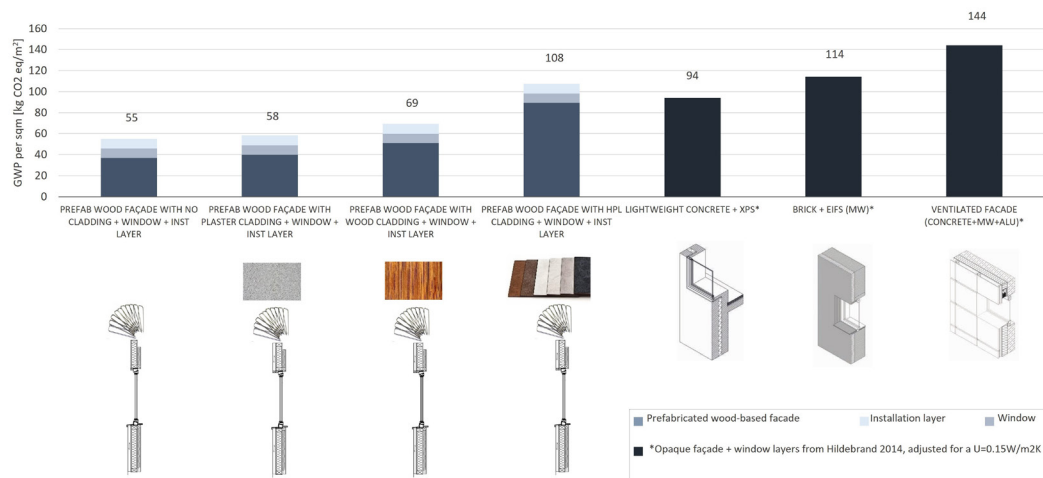
FIG. 8 Global Warming Potential (GWP) per square metre for total life cycle of different multi-layer opaque façade layers (U=0.15W/m 2 K) which include a window. Total Life Cycle Analysis results for Production, Maintenance, and End of Life Phases.
