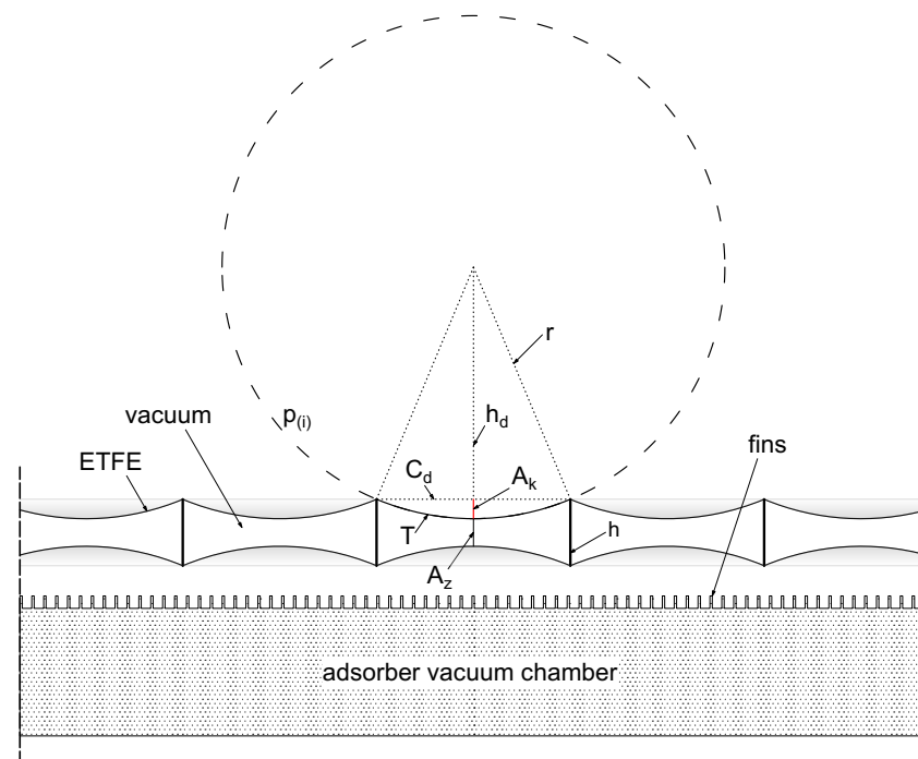
FIG. 11 Calculation sketch for the grid size
