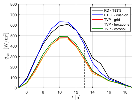
FIG. 18 Comparison RD-T83% with ETFE cushion and EVP with grid/ hexagons/ Voronoi structure aligned to SSE
