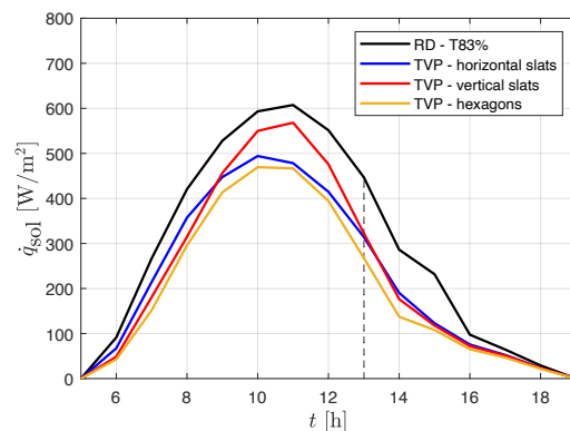
FIG. 19 Comparison RD-T83% with EVP with horizontal and vertical slats and with a hexagon structure aligned to SSE
