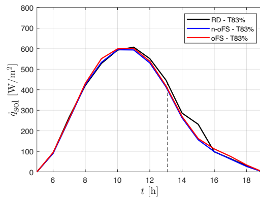
FIG. 16 Comparison RD-T83% with n-oFS and oFS aligned to south-southeast
