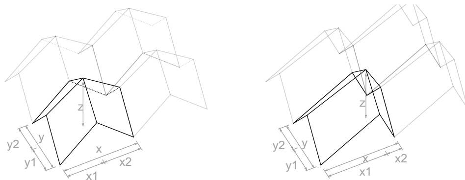
FIG. 9 Optimization method for the isometric folding structure, design/approach based on (Klett, 2013)
