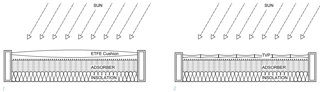
FIG. 10 Top section of the adsorber element with ETFE cushion (left) and transparent vacuum panel (right)
