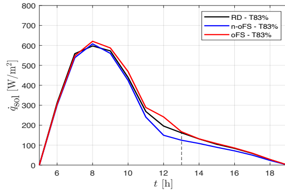
FIG. 17 Comparison RD-T83% with n-oFS and oFS aligned to east
