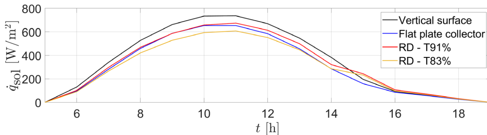
FIG. 13 Solar gains of a vertical surface, flat plate collector, reference design with solarglass T91% and reference design with double glazing T83%
