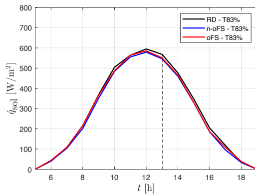
FIG. 15 Comparison RD-T83% with n-oFS and oFS aligned to south
