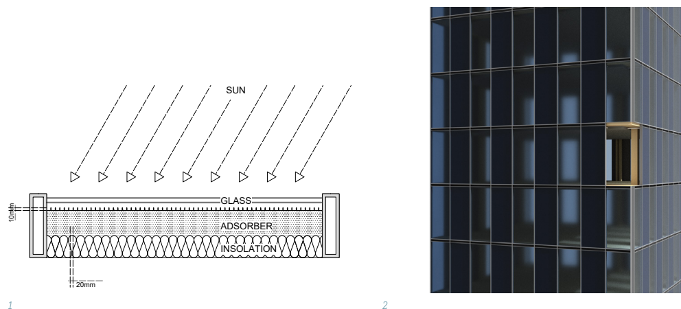
FIG. 5 [1] Top section view adsorption element with reference design, [2] Example of a façade integration of the reference design
