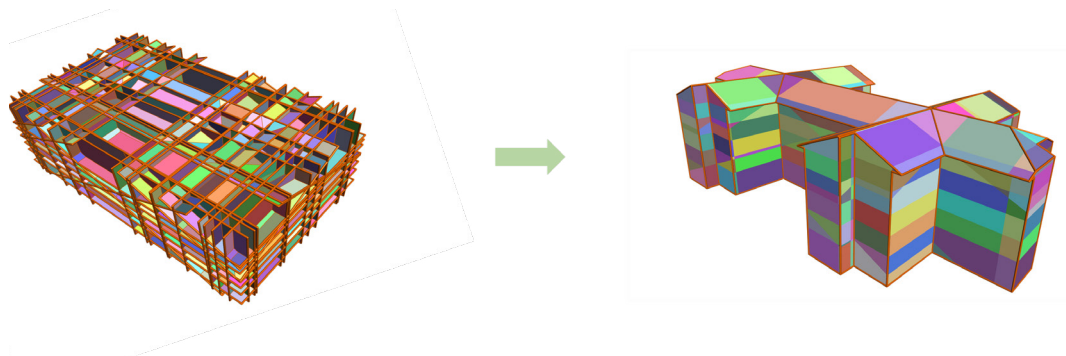
FIG. 3 PolyFit Result: Face Candidates (left) and selected face candidates (right)
