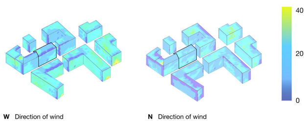
FIG. 4 Wind facade pressure analysis, west and north directions of wind, June-August; 11am – 4 pm (Larikova I., 2021)
