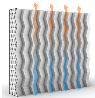
FIG. 8 Thermal air flow through the folded structure
