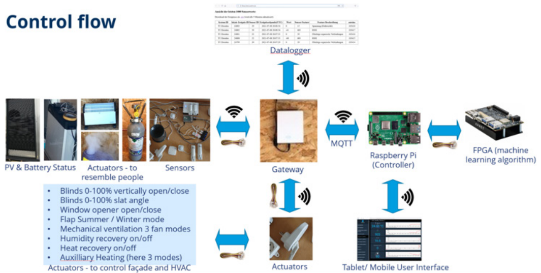
FIG. 10 Control concept of the self-learning PRÄKLIMA façade
