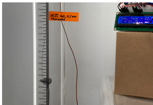
FIG. 5 Testing of the SMA-behavior under maintained and supervised temperature conditions
