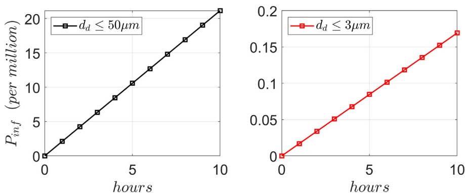
Fig. 21. Long exposure probability of infection. Left: considering all simulated droplets (up to 50 μm). Right: considering only droplets of 1 and 3 μm.
