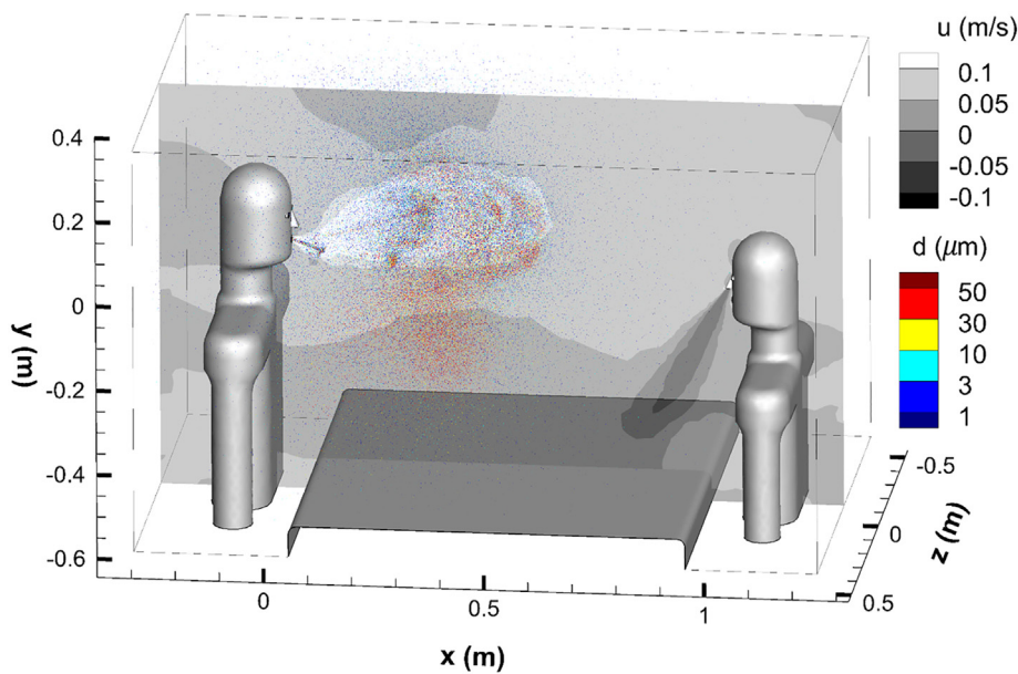
Fig. 15. Simulation of a conversation across a dining/meeting table. The male (left) is infected with SARS-CoV-2, speaks for 15 s followed by 45 s of breathing. The female (right) breathes during the entire simulation. The horizontal velocity contours are shown in the plane z = 0 , while the droplets are plotted over the full simulated volume, delimited by the black dashed-lines.
