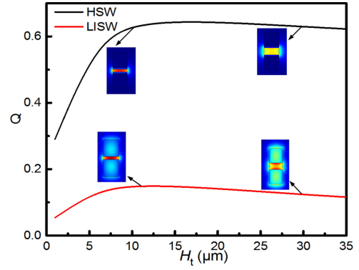
Fig. 3. Confinement factor ( Q ) of HSW (or LISW) as a function of the height of low-index layer ( H_t ).
