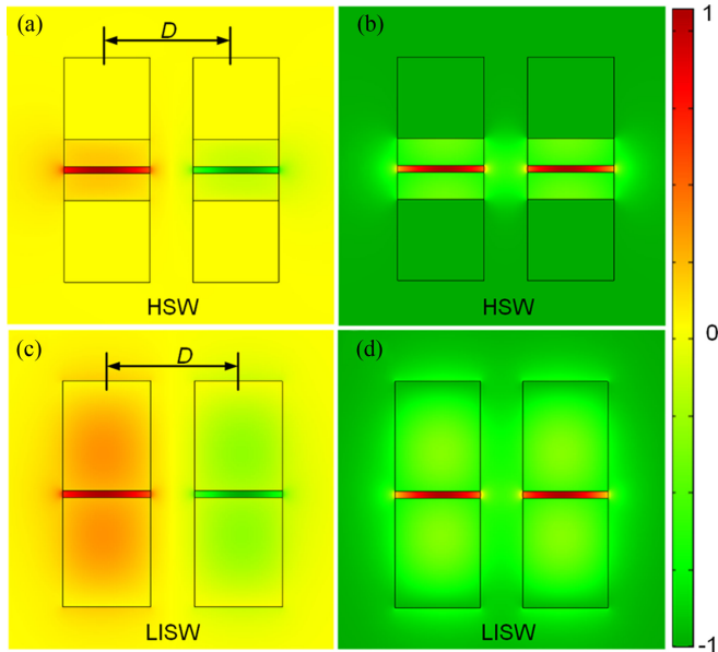
Fig. 5. The E_y field distributions of (a) the anti-symmetric two HSWs; (b) the symmetric two HSWs; (c) the anti-symmetric two LISWs and (d) symmetric two LISWs with a distance of D = 30 \mu\text{m} .
