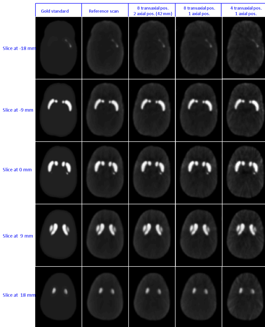
Figure 6. Comparison of the DaTscan image slices from the gold standard (the digital phantom), the reference scan (simulated full brain scan with oversampling), the DaTscan acquired with two axial positions combined with eight transaxial positions (distance between two axial positions is 42 mm), the scan with one axial position combined with eight transaxial positions, and the scan with one axial position combined with four transaxial positions. The center of the striatum in axial direction is defined to be at 0 mm. The top row to the bottom row represent the slices from 18 mm underneath the center of the striatum to 18 mm above it. All images have a pixel size and slice thickness of 1.5 mm and are post-filtered with a Gaussian filter of 4 mm FWHM. The concentration ratio in striatum and background compartment is 8:1. The Colormap is set from 0 to 8 (intensity normalized to that of the background compartment) for the gold standard images, and from 0 to 2.66 (the maximum intensity in the reference scan) for all the simulated DaTscan images. A full overview of the DaTscan images for all the tested sampling sequences using one or two axial positions as well as their difference images from the reference scan are included in the appendix.
