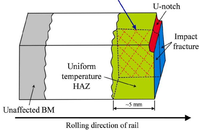
Fig. 3. Testing position diagram of thermal simulation specimen for macroscopic & microscopic characterization. Note: testing position of the BM specimen is consistent with the thermal simulation specimen.
