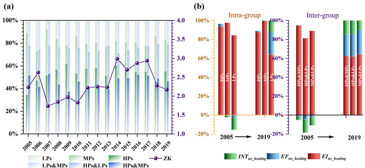
Fig. 7. Imbalance of CI_{no\_heating} at the economy group level.
