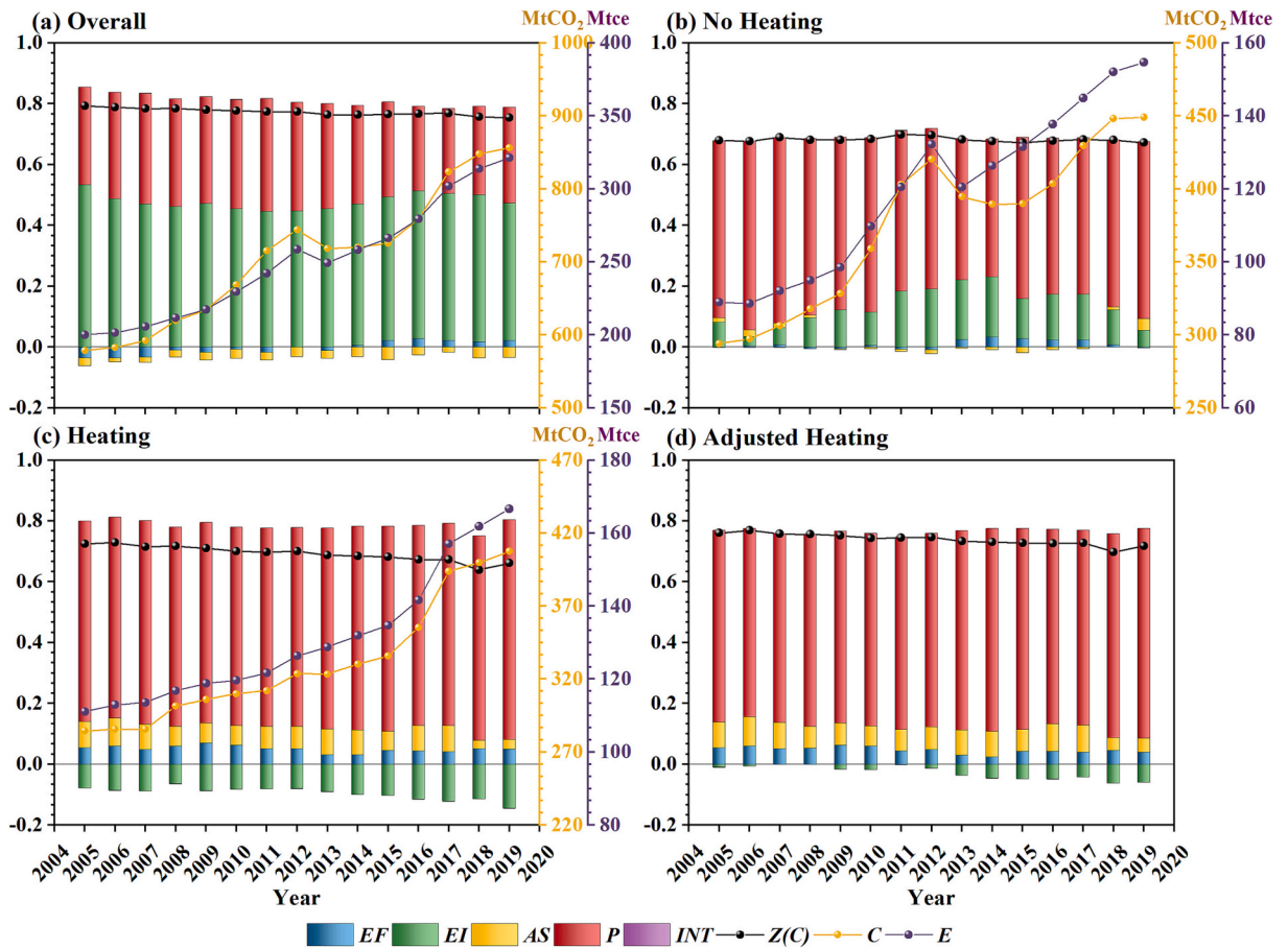
Fig. 3. The imbalance of carbon emissions in URB. (Note: Fig. 3a, b, c, and d represent imbalances in C_{overall} , C_{no\ heating} , C_{heating} , and C_{adj\ heating} , respectively. EF, EI, AS, P and INT represent emission factor, energy consumption unit area, per capita floor area, population and interaction term, respectively.)
