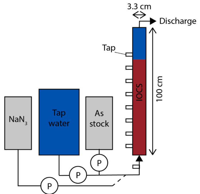
Fig. 1. Schematic overview of the experimental setup, where the P within the circle depict the pumps. During the experiment the column was fed with tap water to which As was added. The tap water and As(III) stock pumps were stopped during microbial inhibition, and only a \text{NaN}_3 solution was fed to the column.
