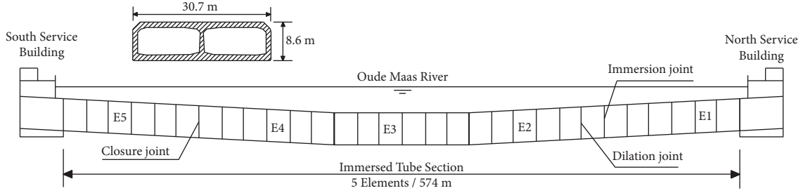
FIGURE 4: Side view of the First Heinenoordtunnel.
