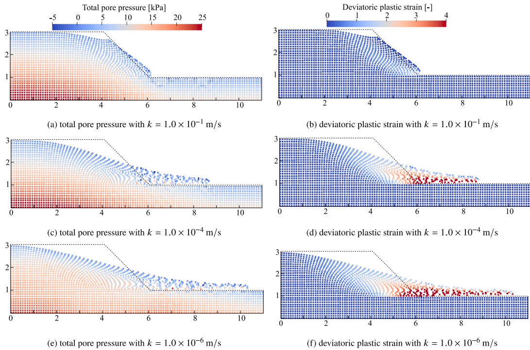
Fig. 13. Configuration after slope failure (at t = 50.0\text{s} ) in water-saturated sand for different values of soil permeability, and associated contours of total pore pressure and deviatoric plastic strain. Results obtained with initial soil dilatancy angle \psi_{ini} = -5^\circ .
