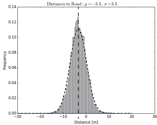
Figure 7: Histogram of a road showing the discrepancy between the OSM geometry (at 0 meters) and the mean of the distances of the samples (at -3.3 meters—dashed line).
