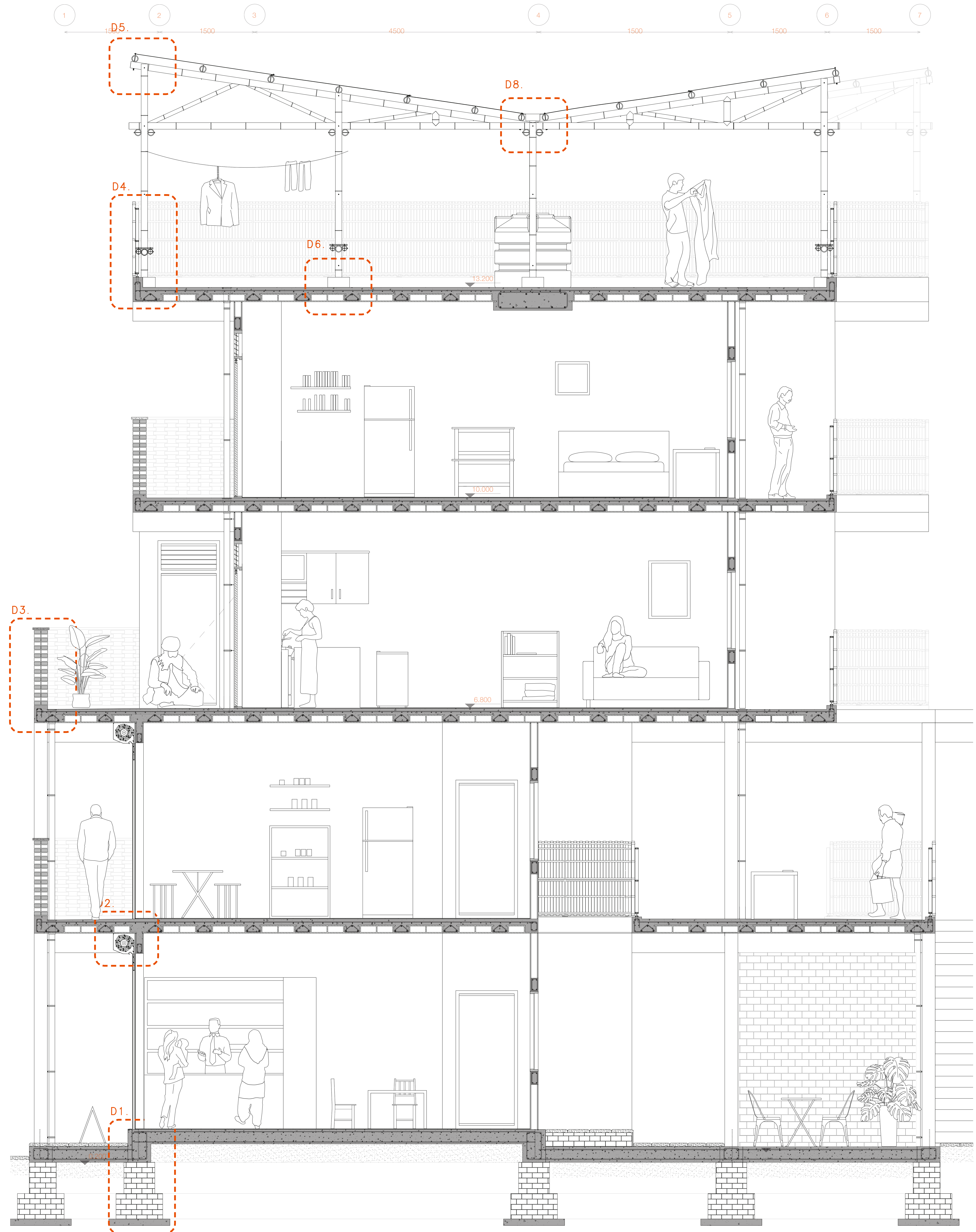
DETAIL SECTION 1:25
