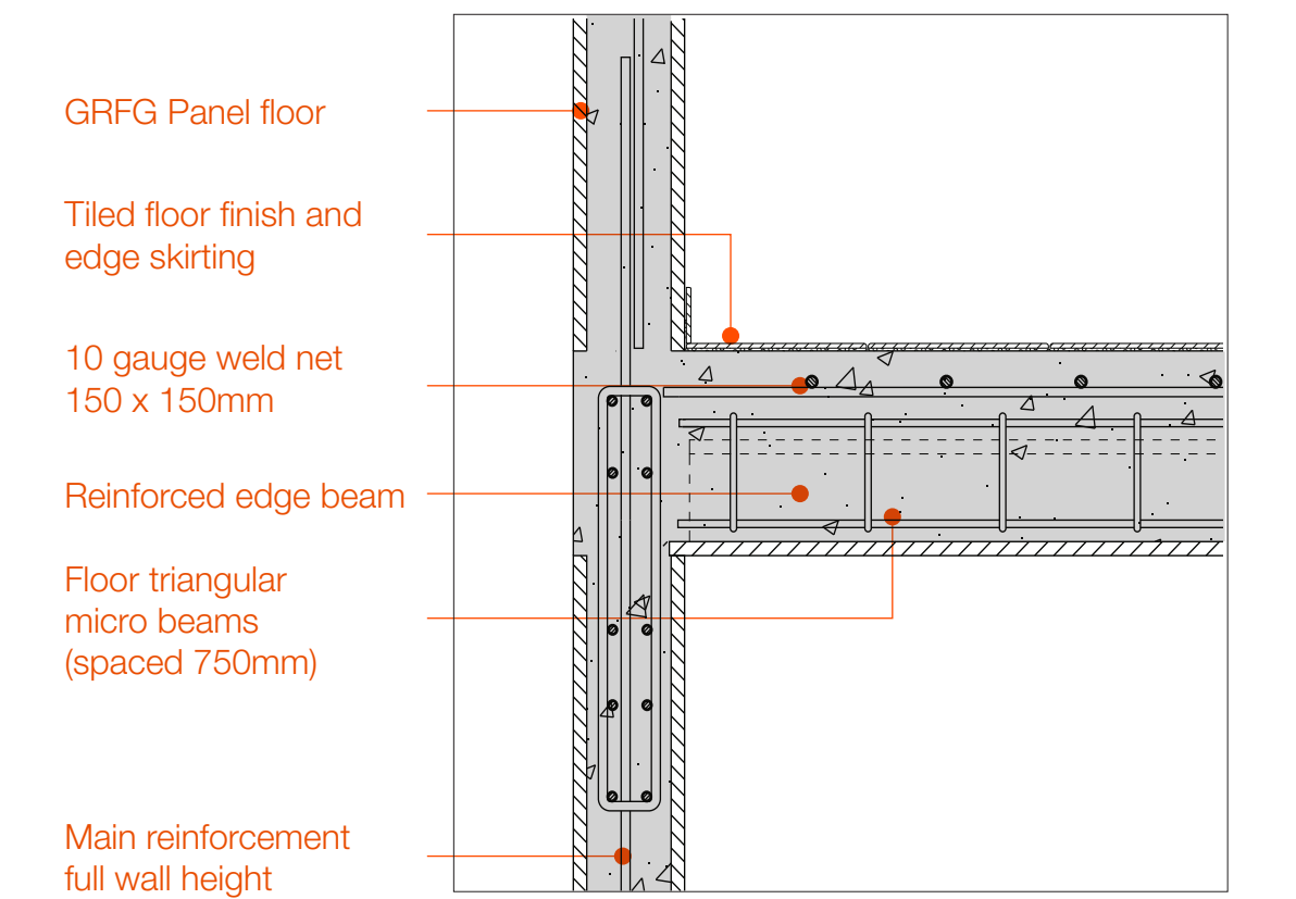
STRUCTURAL D9.
