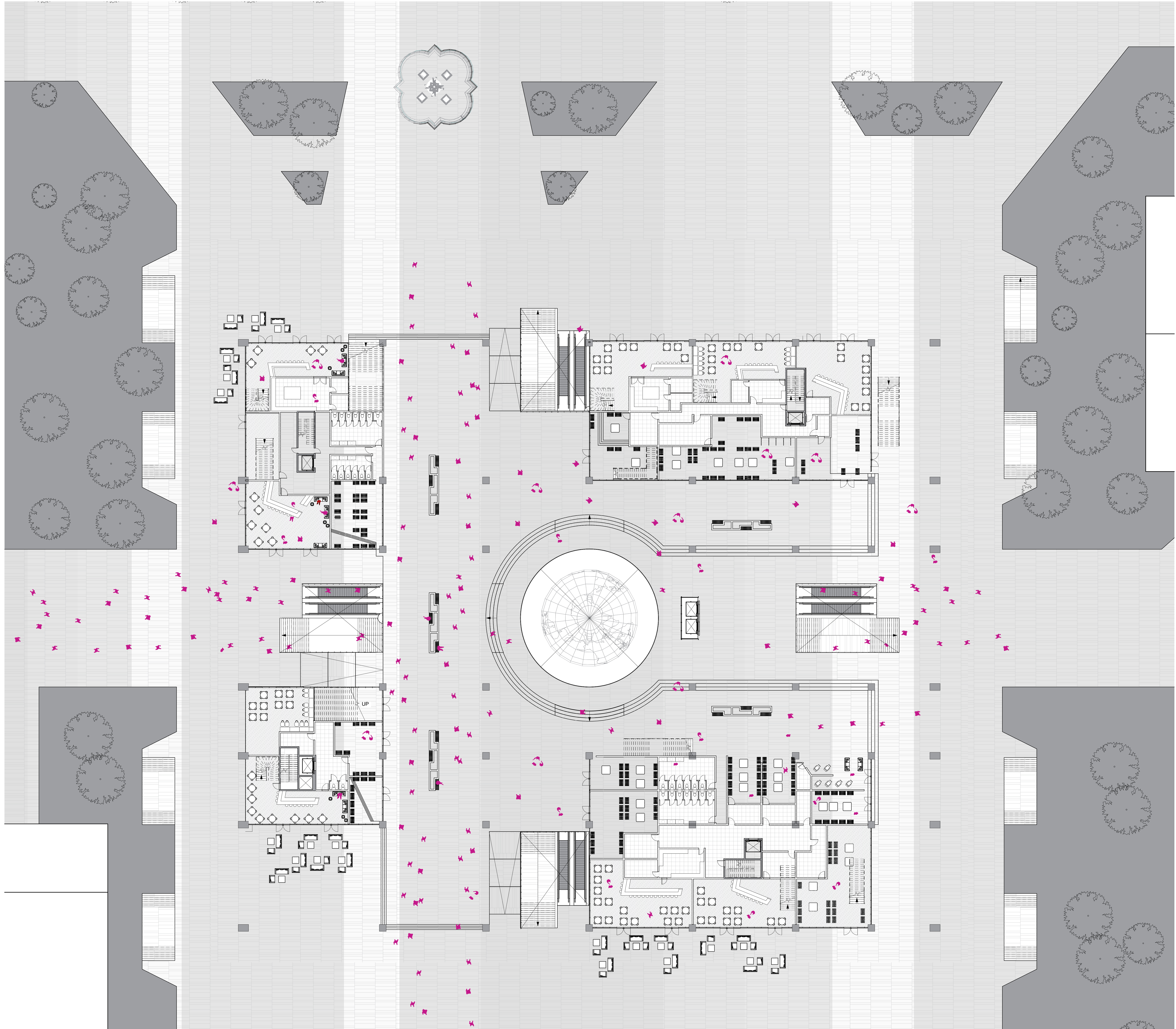
Ground floor +2.5m Scale 1:200
