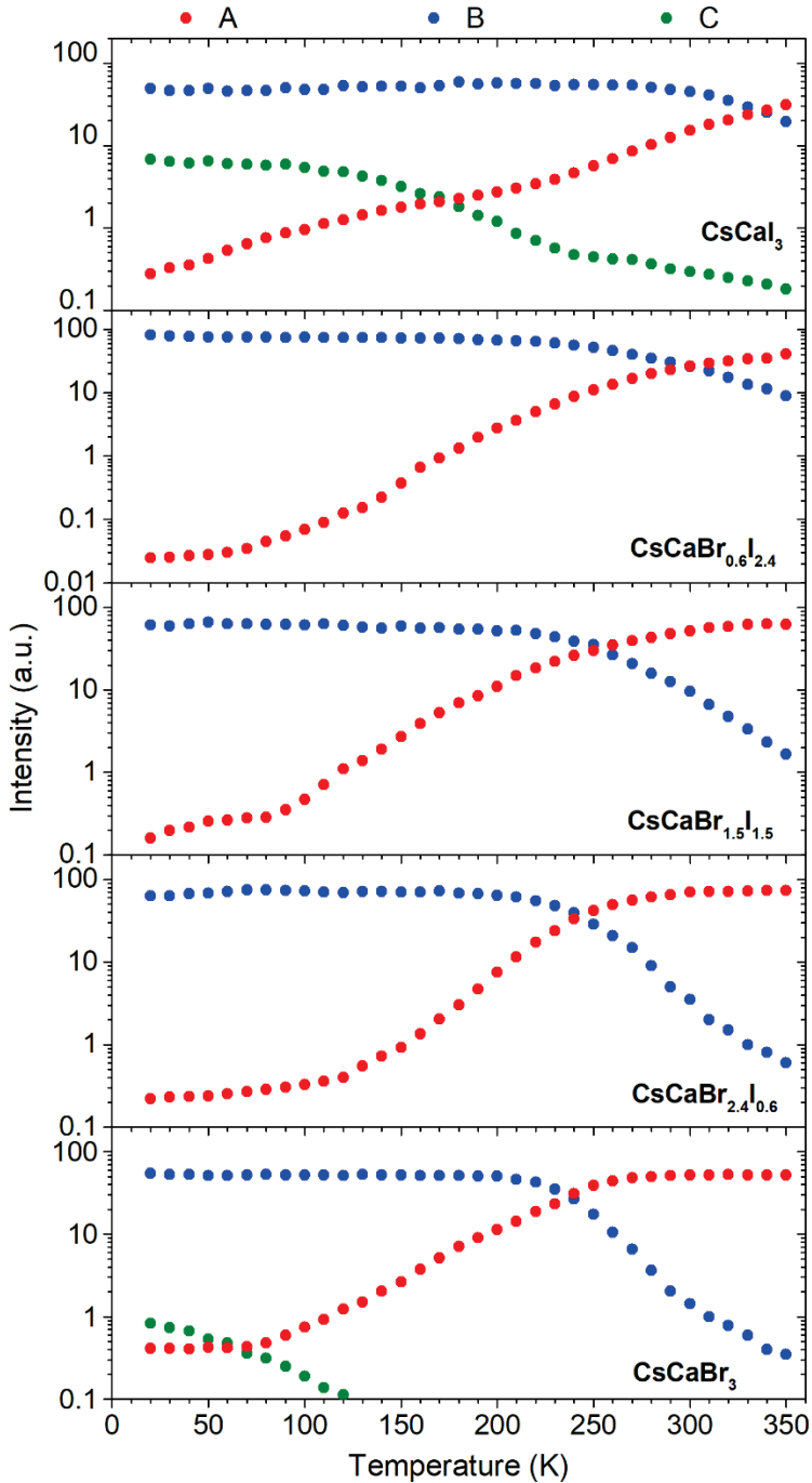
Figure 4.19: Temperature-intensity plots analogous to figure 4.18, but related to the CsCa(Br/I)_3:Tm^{2+} samples.
