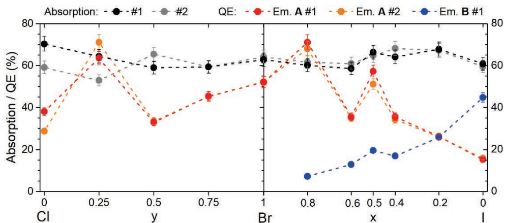
Figure 4.13: Quantum efficiency of the {}^2\text{F}_{5/2} \rightarrow {}^2\text{F}_{7/2} emission A (red) and absorption (black) plotted versus the Br/Cl and Br/I ratio in the samples. For the \text{CsCa}(\text{Br}/\text{I})_3\text{:Tm}^{2+} samples, the QE of ({}^3\text{H}_6, \text{t}_{2g})_{S=3/2} \rightarrow {}^2\text{F}_{7/2} emission B could also be determined (blue). Photoexcitation occurred at room temperature into the ({}^3\text{H}_6, \text{t}_{2g})_{S=1/2} levels. The fluctuation among the QE datapoints was reproduced by a second independent measurement (orange). The absorption remained the same (grey).
