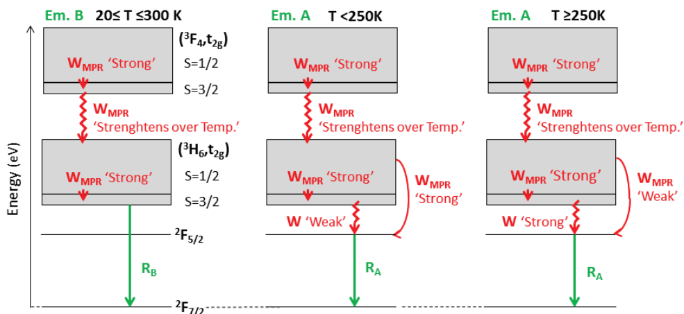
Figure 4.23: Possible explanation for the different excitation spectra as observed in figure 15. The left diagram explains the excitation spectra observed for ( 3 H 6 , t 2g ) S=3/2 → 2 F 7/2 emission B at 20 ≤ T ≤ 300 K. The central diagram explains the excitation spectra of 2 F 5/2 → 2 F 7/2 emission A at T < 250 K using a strong W MPR feeding from the ( 3 H 6 , t 2g ) S=1/2 levels to the 2 F 5/2 level, whereas the right diagram explains this situation at T ≥ 250 K.
