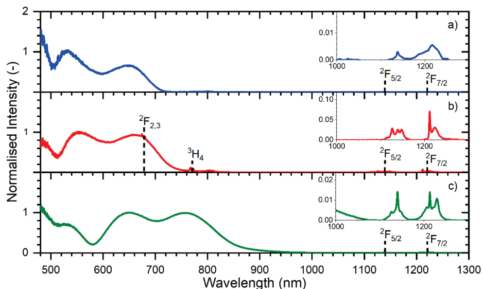
Figure 3.1: The Kubelka-Munk absorption spectra of: a) CaCl 2 :Tm 2+ , b) CaBr 2 :Tm 2+ , and c) CaI 2 :Tm 2+ as normalised on the ( 3 H 6 , t 2g ) absorption band of Tm 2+ . The related Tm 3+ absorption peaks and the Tm 2+ absorption bands and peaks are indicated by their levels. The measurements were performed using a Bruker Vertex 80v with Si and InGaAs photodiode detectors and a Pike Optics EasiDiff diffuse reflectance tool.
