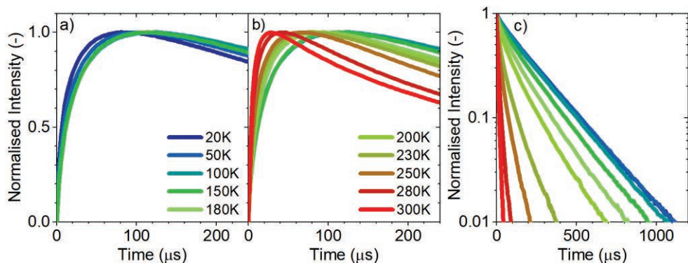
Figure 5.15: The time resolved spectra showing the risetime phenomena as present in the decay curves of {}^2\text{F}_{5/2} \rightarrow {}^2\text{F}_{5/2} emission A (ab) and the decay curves of {}^3\text{H}_6, t_{2g} s=3/2 \rightarrow {}^2\text{F}_{7/2} emission B (c) in sample S7 at different temperatures. The time-resolved spectra were acquired using pulsed laser excitation at 410 nm
