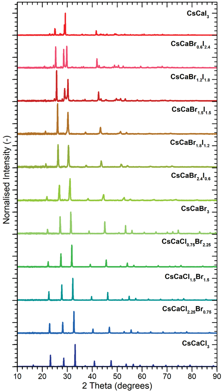
Figure 4.1: Powder X-ray diffraction patterns of the CsCa(Cl/Br)_3:Tm^{2+} and CsCa(Br/I)_3:Tm^{2+} samples at room temperature. The corresponding crystallographic data are summarised in table 4.1.
