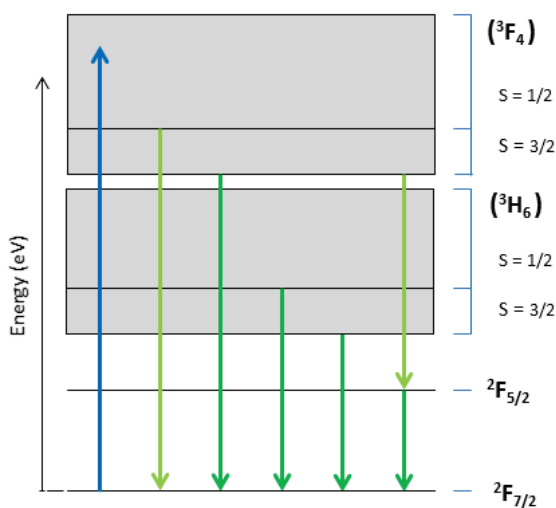
Figure 6.1: Energy level diagram of a typical Tm^{2+} -doped halide with the two lowest energy 4f^{12}5d^1 -levels: (^3F_4) and (^3H_6) . Both levels are split into spin-allowed ( S=1/2 ) and spin-forbidden ( S=3/2 ) states. The latter are positioned at relatively lower energies. Also drawn are the (^2F_{5/2}) 4f^{13} excited state and (^2F_{7/2}) 4f^{13} ground state. The various Tm^{2+} emissions are indicated by green arrows. The light green arrows represent 'rarely' observed Tm^{2+} emissions, such as the (^3F_4)_{S=1/2} \rightarrow ^2F_{7/2} emission, which has up to now only been perceived in CsCaI_3:Tm^{2+} [2,3, chapter 5], and the (^3F_4)_{S=3/2} \rightarrow ^2F_{5/2} emission that can be found in CsCaX_3:Tm^{2+} ( X = Cl, Br, I ) [2, 4, chapter 5] and NaY:Tm^{2+} ( Y = Cl, Br ) [chapter 2]. The (^3H_6)_{S=1/2} \rightarrow ^2F_{7/2} emission is almost always absent in Chloride compounds and up to now has only been reported in BaCl_2:Tm^{2+} . [5]
