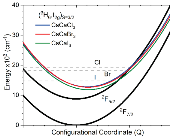
Figure 4.21: Configurational coordinate diagram revealing the \text{Tm}^{2+} {}^2\text{F}_{5/2} , {}^2\text{F}_{7/2} and ( {}^3\text{H}_6, t_{2g})_{S=3/2} State parabolas. The latter ones are drawn for \text{CsCaX}_3:\text{Tm}^{2+} ( X = \text{Cl, Br, I} ) using the information in Appendix B. Note: all state parabolas are drawn here with equal elastic force constant.
