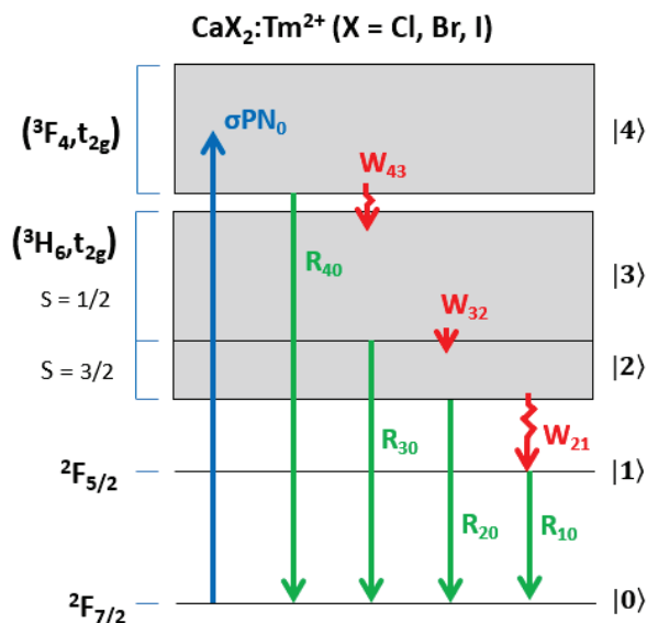
Figure 3.6: Schematic energy level diagram for \text{CaX}_2:\text{Tm}^{2+} upon exciting into the ({}^3F_4, t_{2g}) levels (blue arrow). At 20 K up to four distinct \text{Tm}^{2+} emissions are observed. These radiative transitions are indicated by the green straight arrows R_{ij} , while non-radiative quenching transitions W_{ij} are indicated by the red curly arrows. Here, index i refers to starting level and j the closing level.
