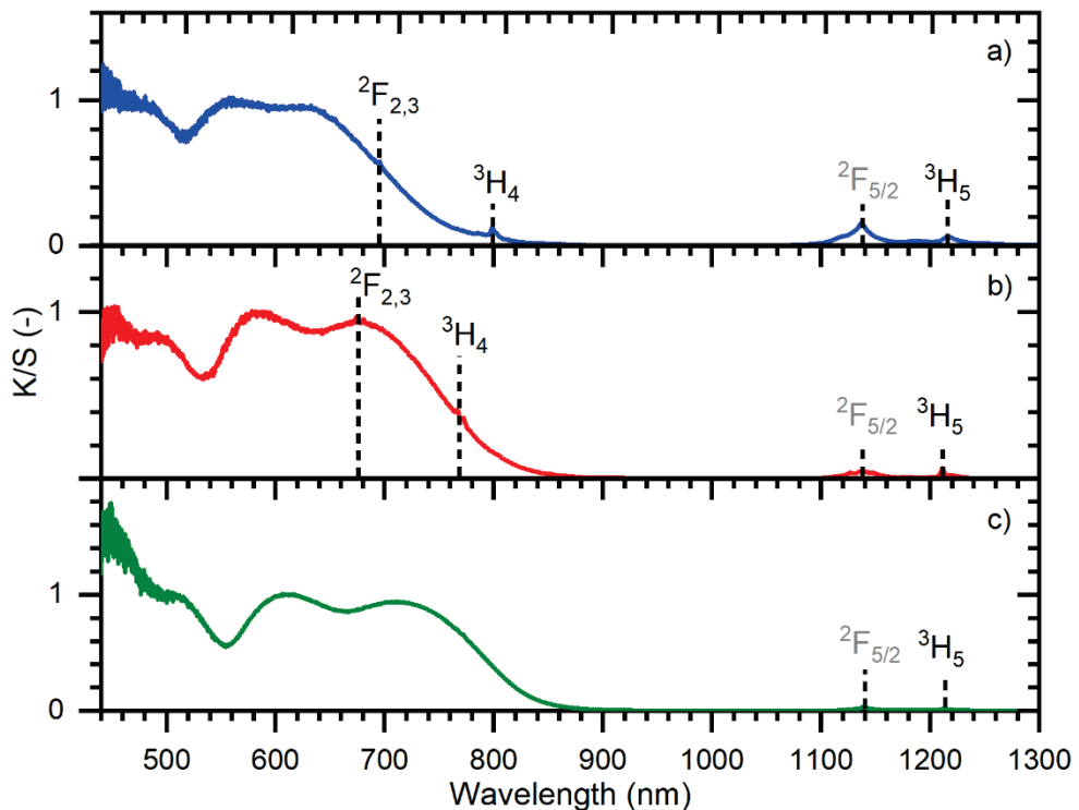
Figure 2.2: The room temperature Kubelka-Munk absorption spectra of: a) \text{NaCl}:\text{Tm}^{2+} , b) \text{NaBr}:\text{Tm}^{2+} , and c) \text{NaI}:\text{Tm}^{2+} . The spectra are normalised on the \text{Tm}^{2+} \ (^3H_6, t_{2g})_{s=1/2} absorption band positioned between 560-600 nm. The absorption peaks of \text{Tm}^{2+} and \text{Tm}^{3+} are labelled and respectively indicated in grey and black.
