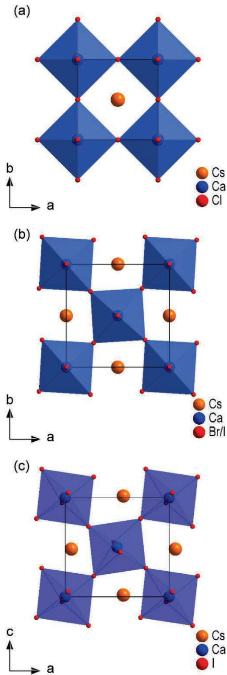
Figure 4.2: Crystal structures of (a) CsCaCl 3 , (b) CsCaBr 1.2 I 1.8 , and (c) CsCaI 3 that respectively adopt the structures of CaTiO 3 , NaNbO 3 , and GdFeO 3 type perovskites.
