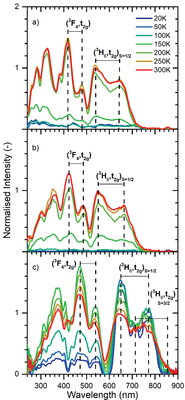
Figure 3.3: Normalised excitation spectra of: a) \text{CaCl}_2:\text{Tm}^{2+} , b) \text{CaBr}_2:\text{Tm}^{2+} and c) \text{CaI}_2:\text{Tm}^{2+} as acquired on the \text{Tm}^{2+} {}^2F_{5/2} \rightarrow {}^2F_{7/2} 4f^{13} \rightarrow 4f^{13} emission at 1140 nm and for different temperatures. The spectra are normalised on the LS ({}^3H_6, t_{2g})_{S=1/2} band at 300 K.
