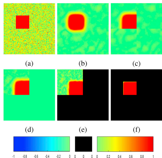
Fig. 5. Normalized weight maps of the various models for the 2D synthetic experiment. The black color indicates weights that are exactly zero. (a) linear SVM; (b) SVM + SR; (c) SVM + SAR; (d) group lasso SVM + SAR using grouping A and low sparsity weight; (e) group lasso SVM + SAR using grouping A and high sparsity weight; (f) group lasso SVM + SAR using grouping B and high sparsity weight.
