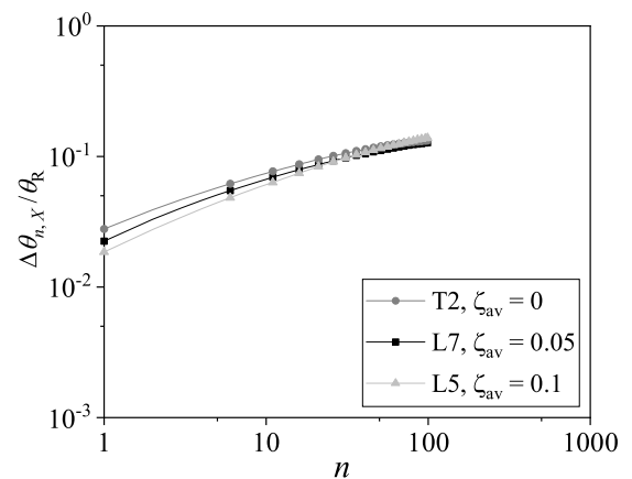
Fig. 16. Influence of average load during cycling \zeta_{av} on the accumulated normalised pile rotation along the X direction — D_r = 70\% .
