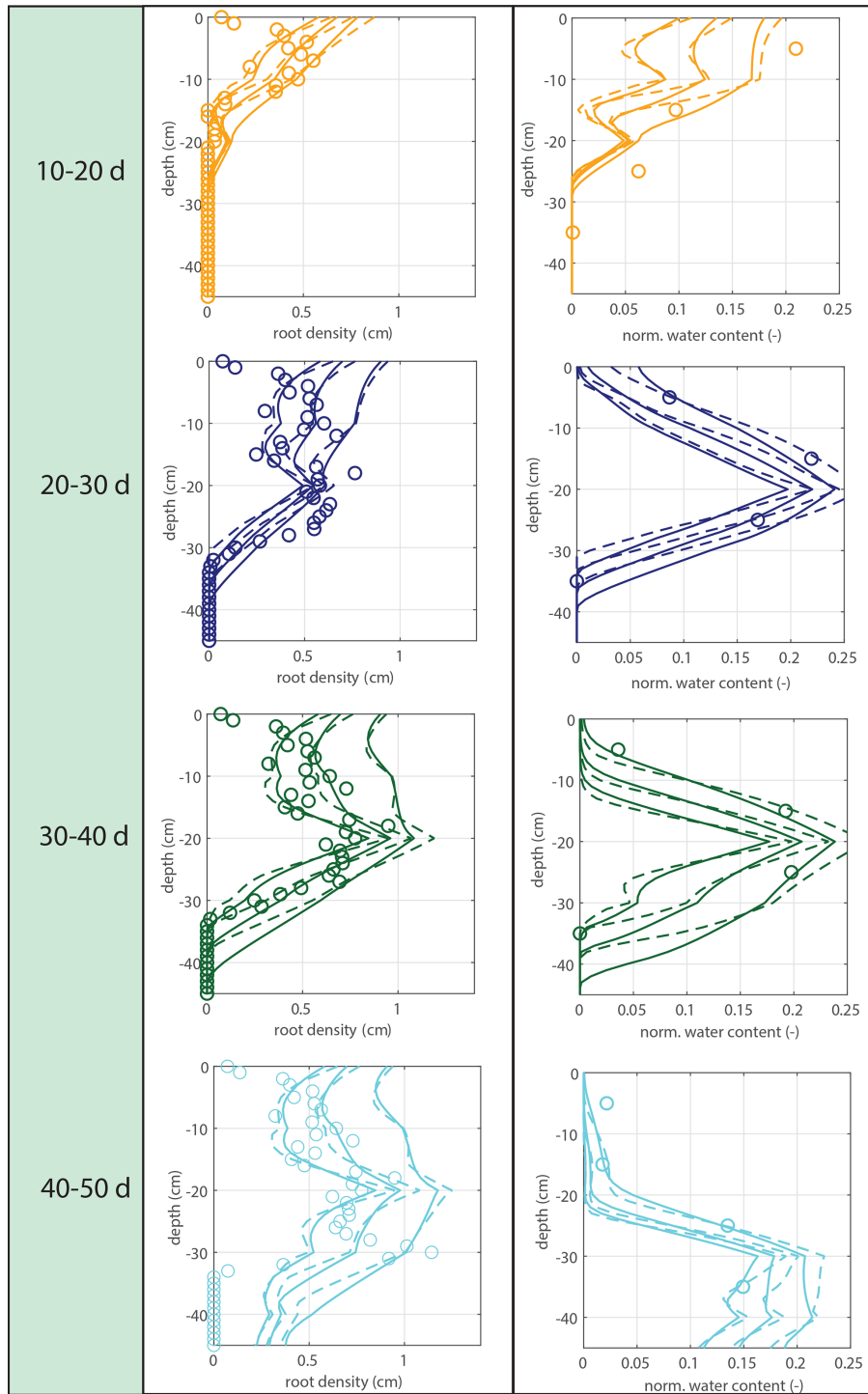
Figure 14. Comparison of results for loamy sand (solid lines) and sandy loam (dashed lines) for three different values for u_2 ( 0.6 \times 10^{-2} , 1.2 \times 10^{-2} , and 2.4 \times 10^{-2} \text{ mL cm}^{-1} \text{ h}^{-1} ).
