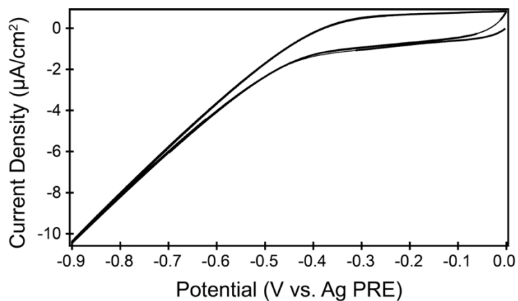
Figure A2.2 CV of ZnO QD film scanned outside of the glove box in an electrochemical cell containing 0.1 M \text{LiClO}_4 in ACN.
