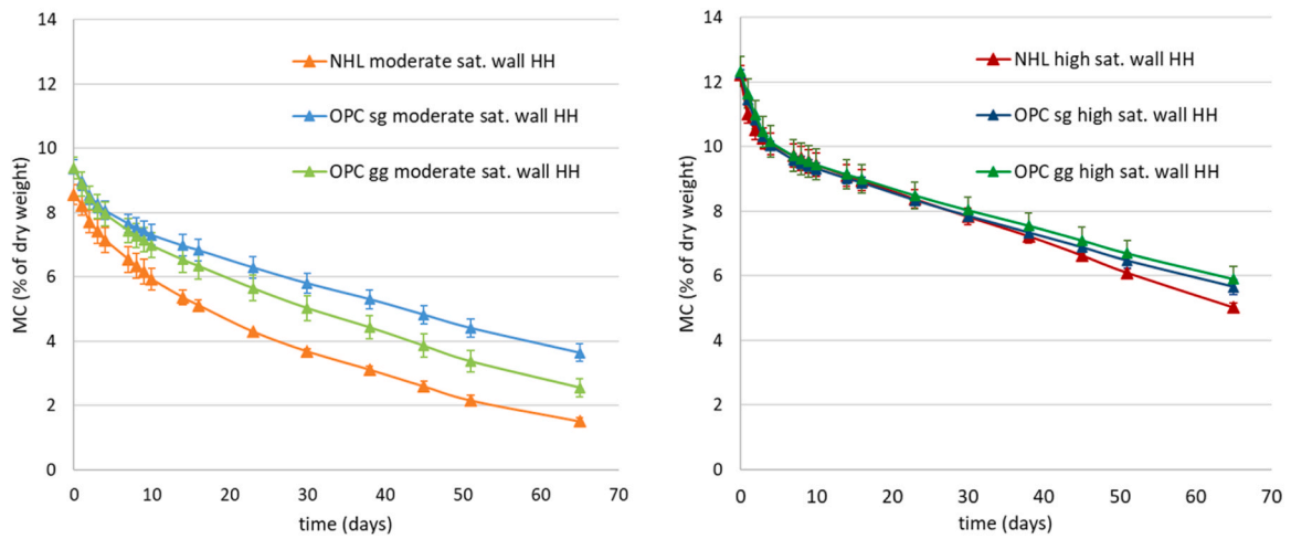
Fig. 11. Drying curves of masonry walls treated with water repellent and subsequently repointed (HH), starting at moderate (left) and high (right) saturation. Each line is the average of measurements on 3 specimens, the vertical bars report the standard variation.
