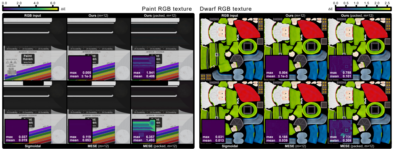
Fig. 11. Unconstrained texture uplifting. We uplift RGB textures and render under D_{65} . We show output for our method ( m = 12 coefficients), a low-bit packed variant, the sigmoidal [Jakob and Hanika 2019] and bounded MESE [Peters et al. 2019]. Mean and maximum \Delta E_{00} are listed for all outputs.
