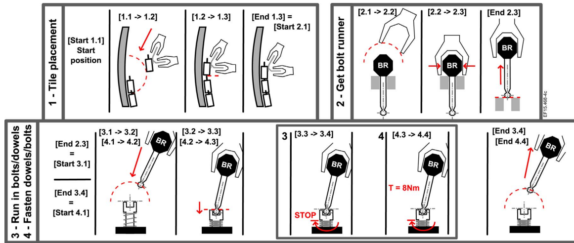
Fig. 4. Schematic representation of the Mascot slave in the remote environment showing the defined state transitions for subtasks ‘1-Tile placement’ (top left), ‘2-Get bolt runner (BR)’ (top right), and ‘3-Run in bolts’ (bottom) and ‘4-Fasten bolts’ (bottom). The states are described in more detail in Table 1.
