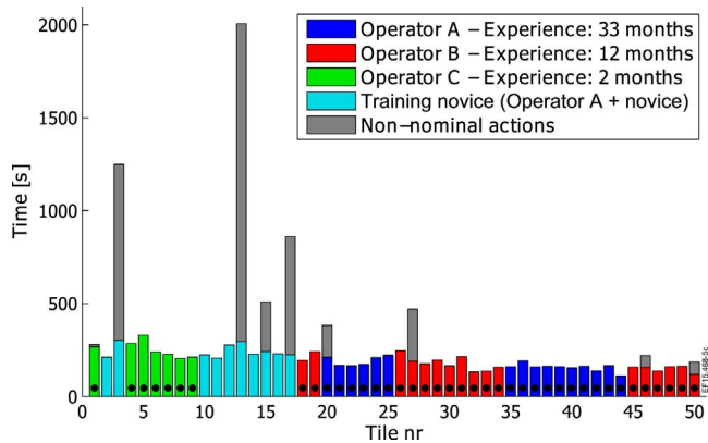
Fig. 5. Task completion time for the installation of 50 tile carriers. The bar colour shows which master-slave operator was on shift. Grey peaks show non-nominal actions. Marked tile installations (●) are performed by fully trained qualified operators and are used for further analysis.
