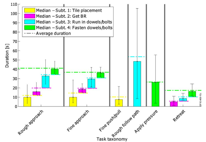
Fig. 10. Analysis phase IIIA. Task completion time is shown for all states (complete task) grouped according to a generalised set of actions (see Table 1 and [25]). The bars show the median duration and are plotted cumulative per generalised action. Bar colours show the corresponding subtasks. The error bars represent the 1st and 3rd quartiles.
