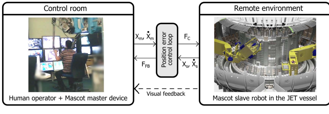
Fig. 1. Schematic representation of the Mascot telemanipulation system at JET. The human operator controls the two arms of the Mascot slave robot (right) by manipulating the two Mascot master arms (left). The master and slave robot are kinematic identical ( 2 \times 6\text{DOF} + \text{grripper} ). The human operator gets visual and haptic feedback ( F_{FB} ) from the environment.
