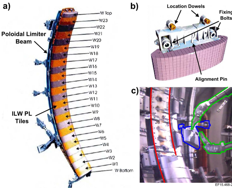
Fig. 2. Analysed maintenance task: 'Install tile to beam' during 'Installation of ITER Like Wall (ILW) Poloidal Limiter (PL) tile carriers'. a) 1 of the 10 Poloidal Limiter Beams in the JET vessel, consisting of 25 tiles. b) ILW PL tile (+/-10 kg). c) A tool interface with two grip features is connected to the tile (highlighted in blue) to allow the two handed placement (see two slave arms highlighted in green). The bolt runner tool is also transported with this tool interface. The target location (PL beam) is highlighted in red. (For interpretation of the references to colour in this figure legend, the reader is referred to the web version of this article.)
