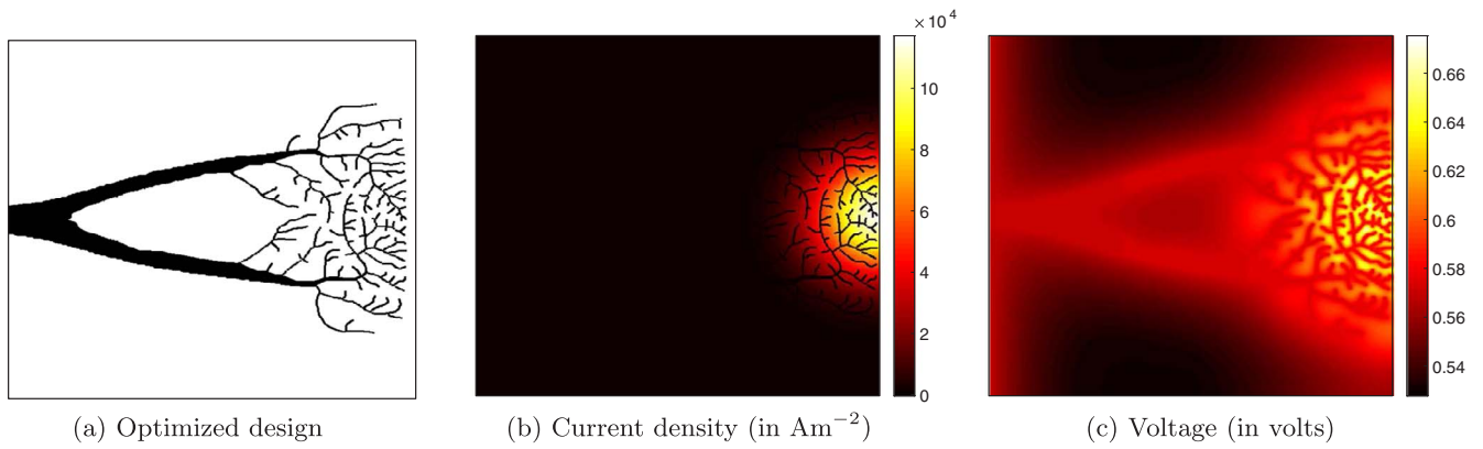
Fig. 11. Optimized design and the current density and voltage distributions for the front side of a solar cell under a Gaussian illumination of an average intensity of 12 suns ( A_0 = 20 ). A uniform temperature profile is chosen with base temperature set to 320 K. The optimal busbar potential V_b and efficiency \eta values are 0.566 volts and 16.846%, respectively.
