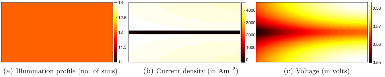
Fig. 4. Uniform illumination profile for 12 suns and the out-of-plane current density and voltage distributions observed in one cell element (1 sun = 1000 W m -2 ).
