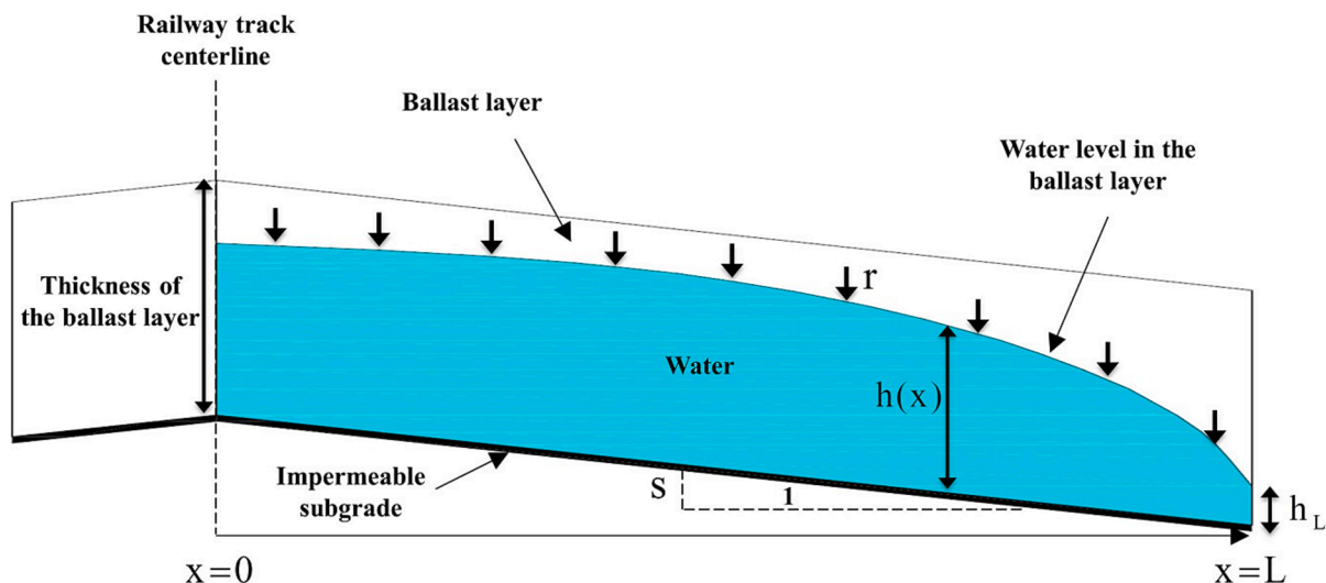
Fig. 6. Schematic cross-section of the ballast layer of the railway track substructure (after [6]).
