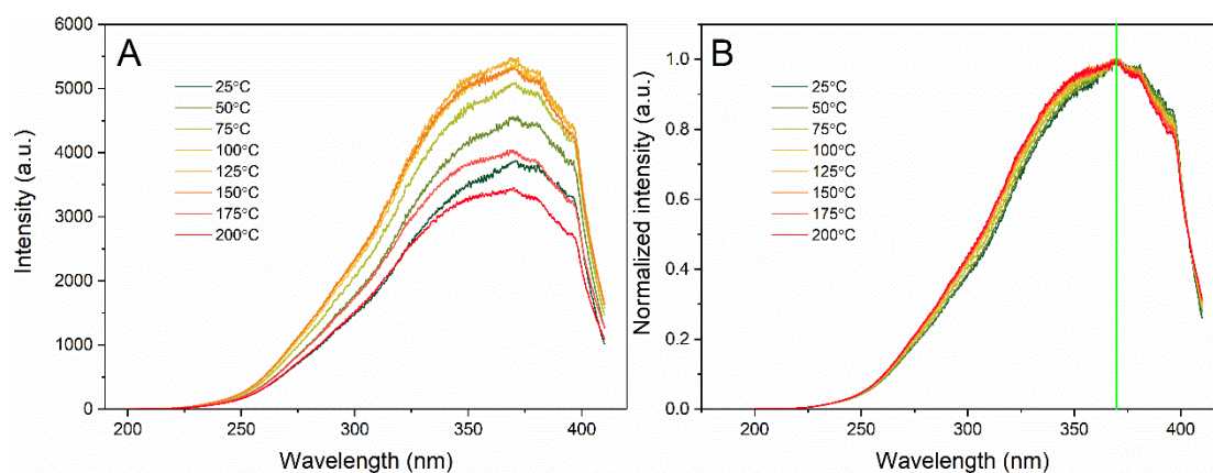
Figure S8. (A) The temperature-dependent excitation spectrum of SB 0.3 PE under the monitoring at 420 nm. (B) The normalized temperature-dependent excitation spectrum. Related to Figure 3.
