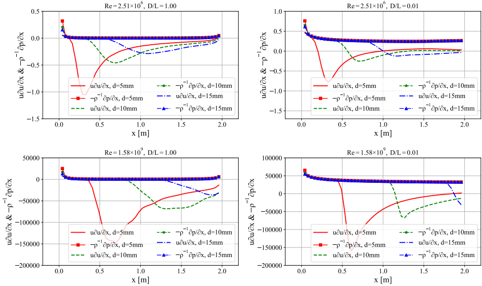
Figure 4.14: Magnitude comparisons of u\partial u/\partial x and -\rho^{-1} \cdot \partial p/\partial x at four conditions (Case information is shown at the top of each sub-graph. The y axis denotes the magnitudes of u\partial u/\partial x and -\rho^{-1} \cdot \partial p/\partial x . The x axis shows the position from the leading edge to trailing edge of the flat plate)
