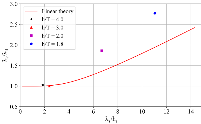
Figure 6.6: The ratio of wavelengths in shallow and deep water ( \lambda_s/\lambda_d ) against the ratio of wavelength and water depth ( \lambda_s/h_s ) based on linear wave theory compared with some CFD results in shallow water
