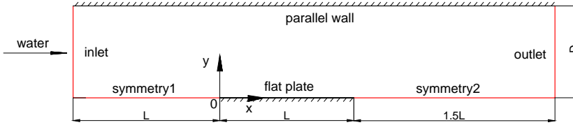
Figure 4.4: Computational domain
