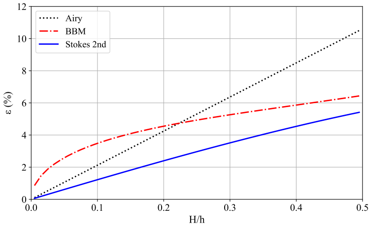
Figure 6.11: Energy dissipation on the bottom over one wavelength ( \epsilon ) against wave height-water depth ratio ( H/h ) for three wave theories ( C_{fb} = 0.1, \lambda/h = 10 )
