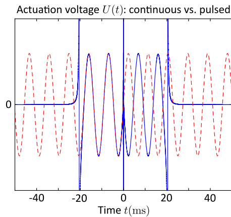
FIG. 2. Comparison of the actuation signal for the second resonant Bessel mode on the LL for an infinitely extended lens using the analytic model (red) and a finite lens radius using the proposed Hankel transform method (blue).
