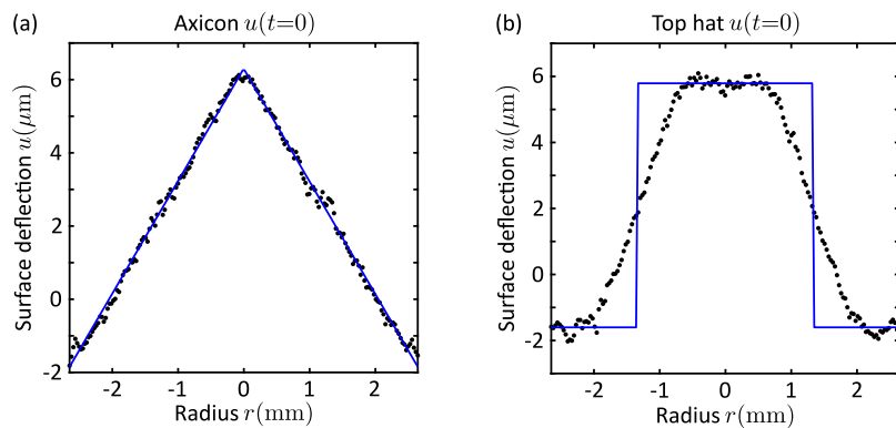
FIG. 6. A pulsed signal is used to design a specific surface shape (blue) and measured interferometrically (black dots) for (a) an axicon and (b) a top hat.
