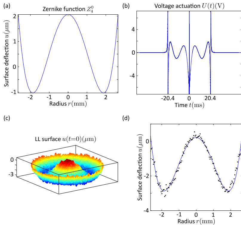
FIG. 5. The primary spherical aberration (a) is transformed into a voltage actuation signal (b). The surface measurement is displayed (c) and a surface profile is shown (d).
