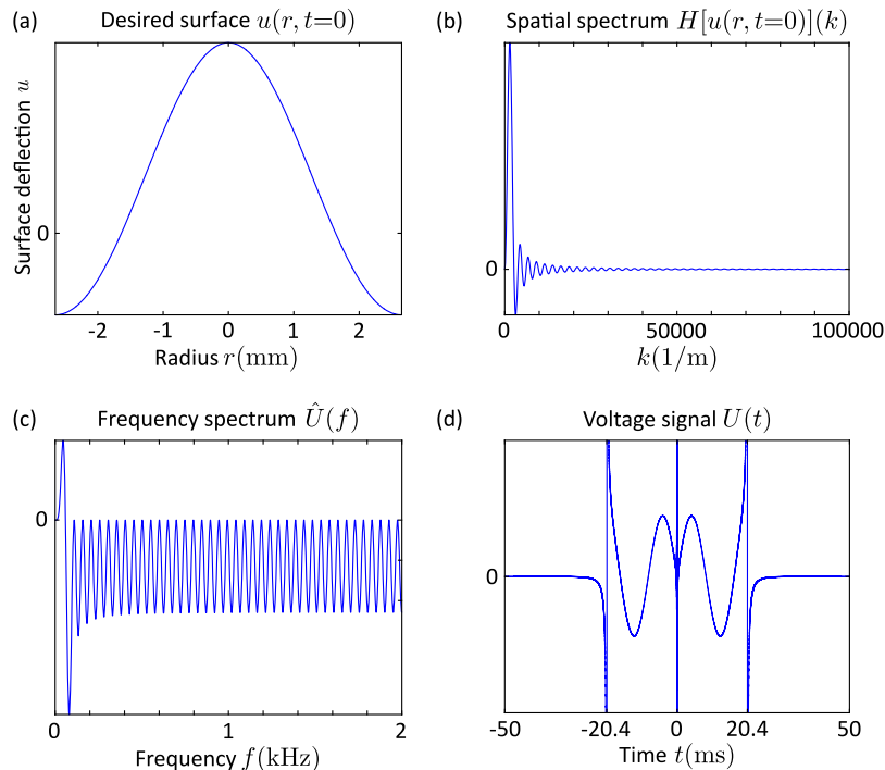
FIG. 1. Illustration of the working principle of the Hankel transform algorithm. The desired surface shape u (here: first Bessel mode) is taken as an input function (a) and converted into its Bessel components H_0 (b). The frequency spectrum of the actuation voltage \hat{U}(f) is displayed in (c) and then Fourier transformed to obtain the voltage actuation signal U(t) (d).
