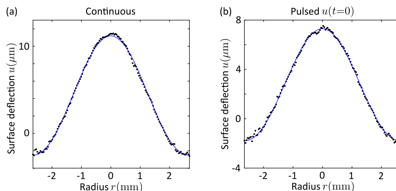
FIG. 4. The Bessel function created in two different ways: (a) by a continuous 59 Hz cosine actuation signal and (b) by a pulsed signal as shown in FIG. 1 (black dots). The theoretical prediction is plotted in blue. Multimedia views: https://doi.org/10.1063/1.5063994.1 ; https://doi.org/10.1063/1.5063994.2
