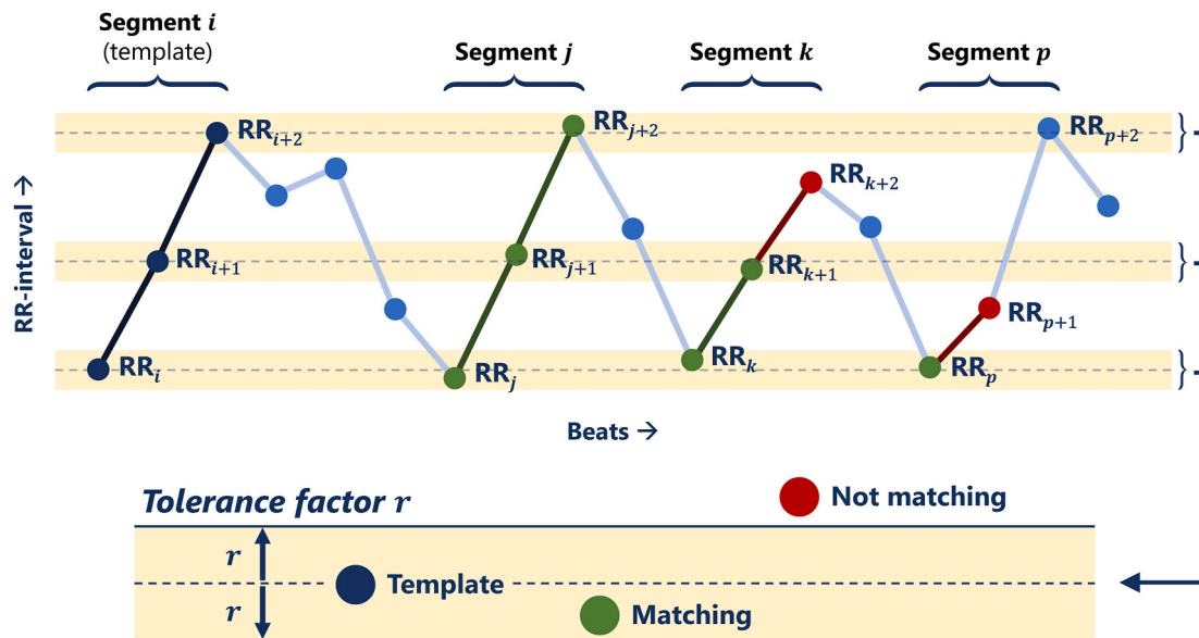
Fig. 5. Schematic visualization of matching used in sample entropy. Segment i is used as a template to compare with segments j, k and p . When setting the prior window length to one RR-interval, hence comparing only the first RR-interval of the segments, all three segments match the template. However, only segments j and k match for the next RR-interval, since RR_{p+1} is below the tolerance range. Increasing the prior window length from one to two RR-intervals results in segment p not matching the template, hence only segments j and k will be tested to match the next RR-interval. In this case, only segment j meets this requirement, as RR_{k+2} is below the tolerance range.
