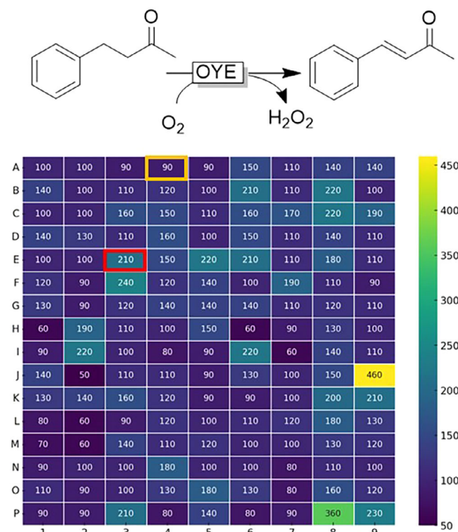
Figure 6. Results from screening the Seqens OYE library for desaturation activity. Conditions: [recombinant "wet" Escherichia coli cells] = 10–20 g/L; 50 mM CHES-NaOH pH 9, 30 ^{\circ} C, 5% v/v DMSO. Emphasized entries: Orange encircled: TsOYE, red encircled: GkOYE; C6: yeast OYE, G6 and N4: bacterial OYE, M4: plant OYE. Numbers shown represent the product concentration relative to the TsOYE sample (A4). Absolute numbers are given in the Supporting Information: Section 2.7.
