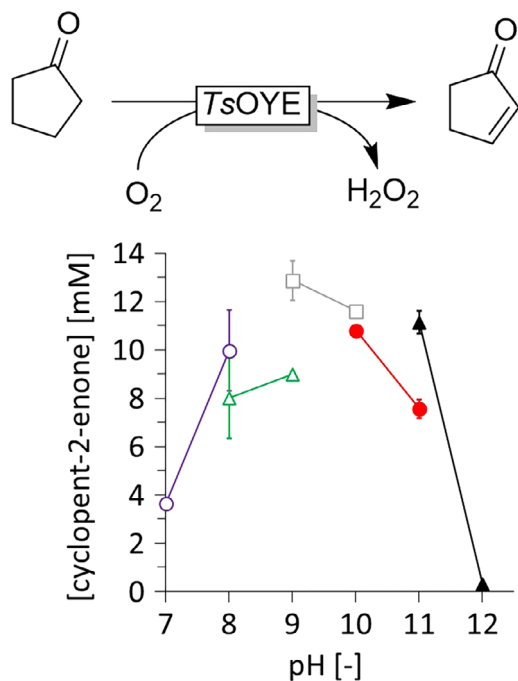
Figure 2. Influence of pH on the product formation of the TsOYE -catalyzed aerobic desaturation of cyclopentanone. Conditions: [cyclopentanone] = 25 mM, [ TsOYE ] = 10 \mu M, 30 ^{\circ} C, 22 h, 50 mM buffer: (○ pink ) MOPS-NaOH (3-( N -morpholino)propanesulfonic acid), (△ green ) Tris-HCl (tris(hydroxymethyl)aminomethane) (12 mM), (□ grey ) CHES-NaOH (2-( N -cyclohexylamino)ethanesulfonic acid), (● red ) CAPS ( N -cyclohexyl-3-aminopropanesulfonic acid), and (▲ black ) PIP (piperazine), 2.5% v/v DMSO.
