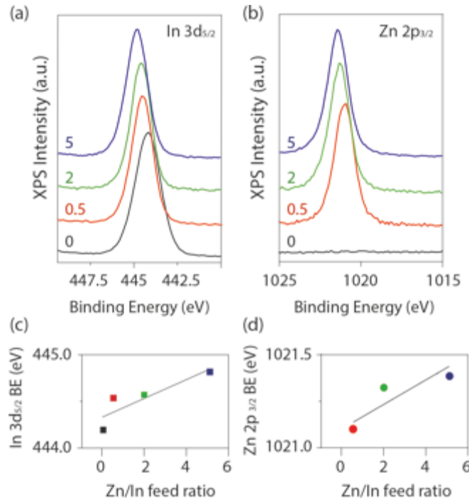
Figure 2- (a-b) In 3d_{5/2} and the Zn 2p_{3/2} XPS spectra for several \text{In}_x\text{Zn}_y\text{P} samples. Each spectrum is labelled with the Zn/In feed ratio. (c-d) The position of In and Zn peaks shifts to higher binding energy values when increasing the Zn/In feed ratio, as summarized in panels c and d.
