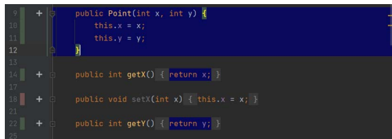
Figure 4: Example of traced code being highlighted.
