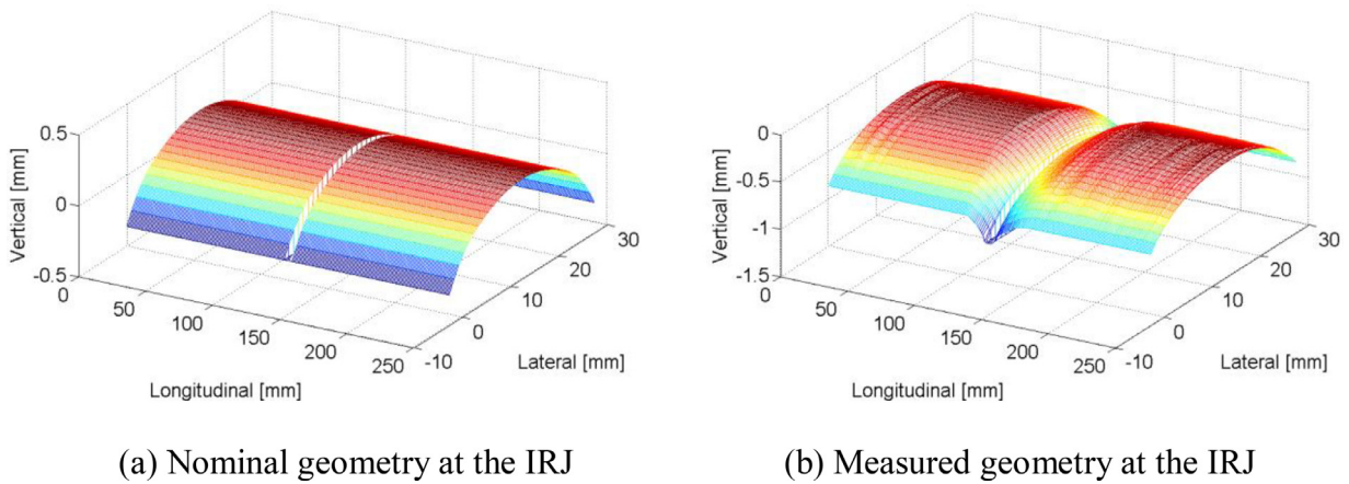
Fig. 3. Applying the realistic geometry to the IRJ (the size of the irregularity is exaggerated) [1].
